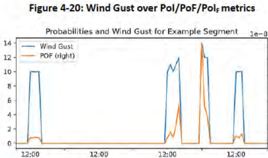
Figure 4 - Top half of SDG&E's Figure 4-20, which shows probability of failure as a function of wind speed.
