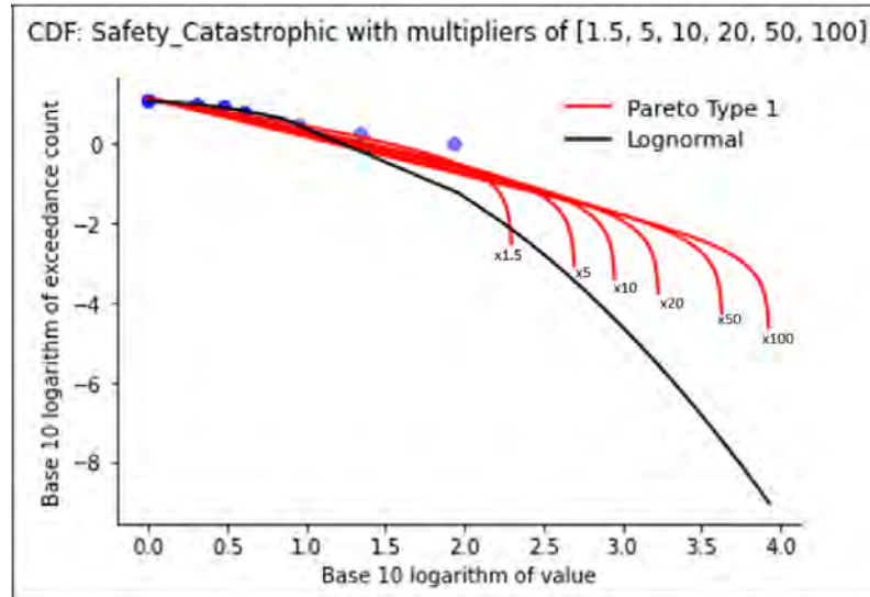
Figure C1 Truncated PD1 and untruncated lognormal distribution fits to wildfire safety consequence data.
