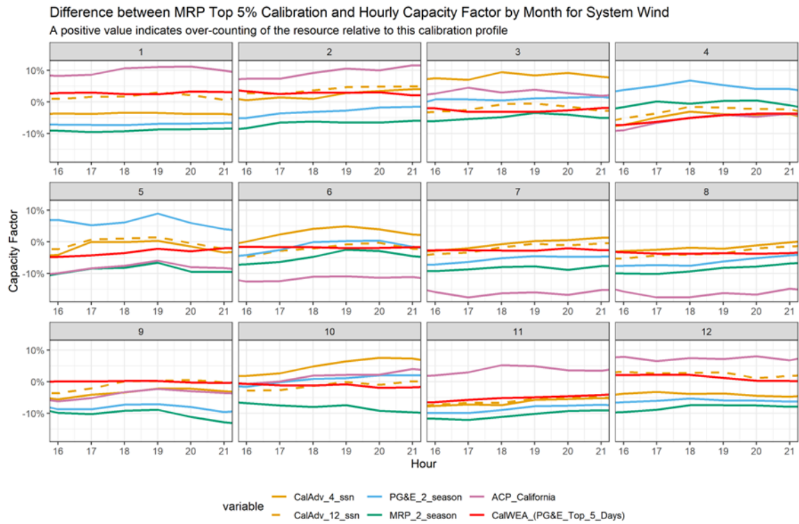
Figure 49: Difference between MRP Top 5% Calibration and Hourly Capacity Factor by Month for System Wind
