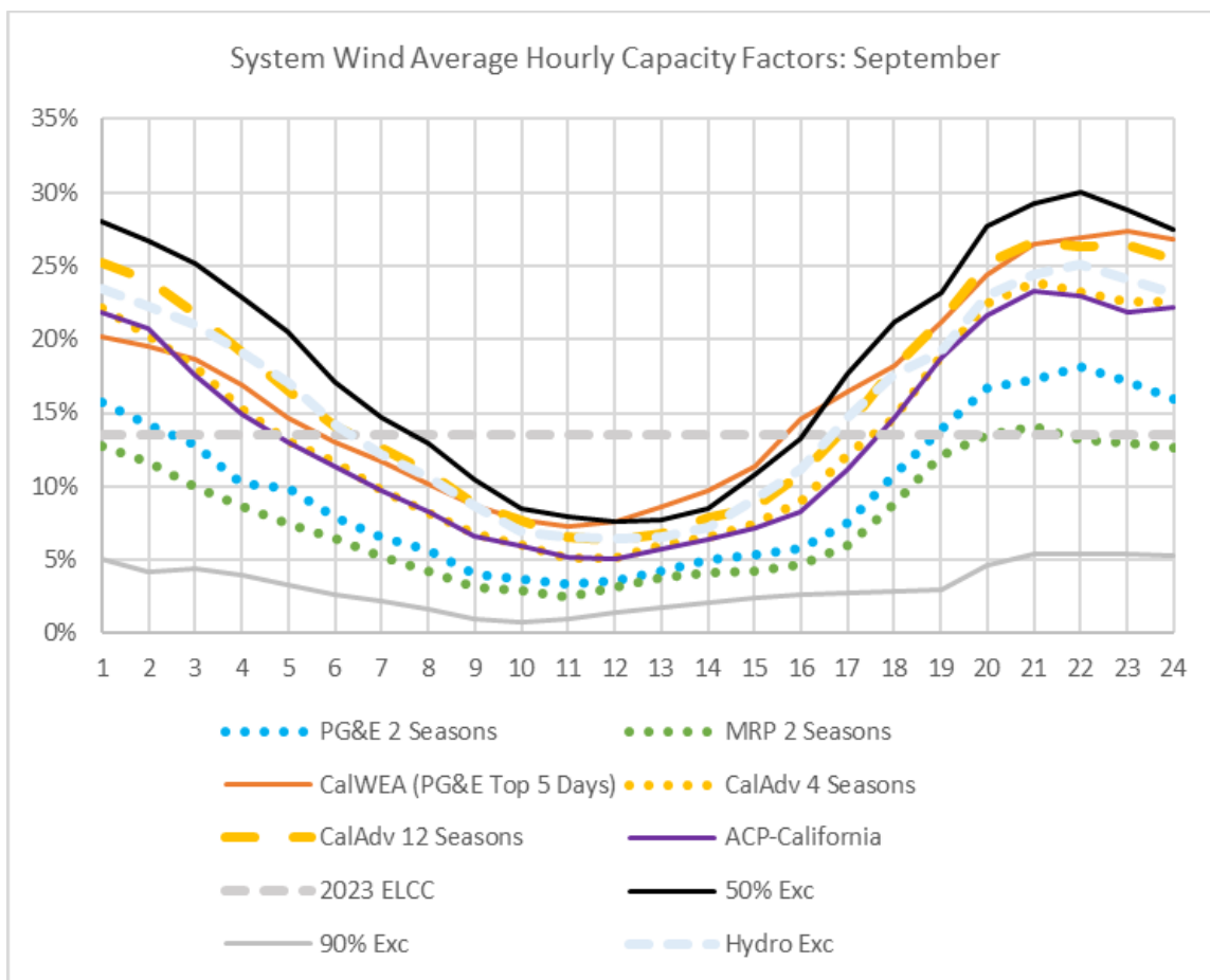
Figure 44: System Wind Average Hourly Capacity Factors: September
