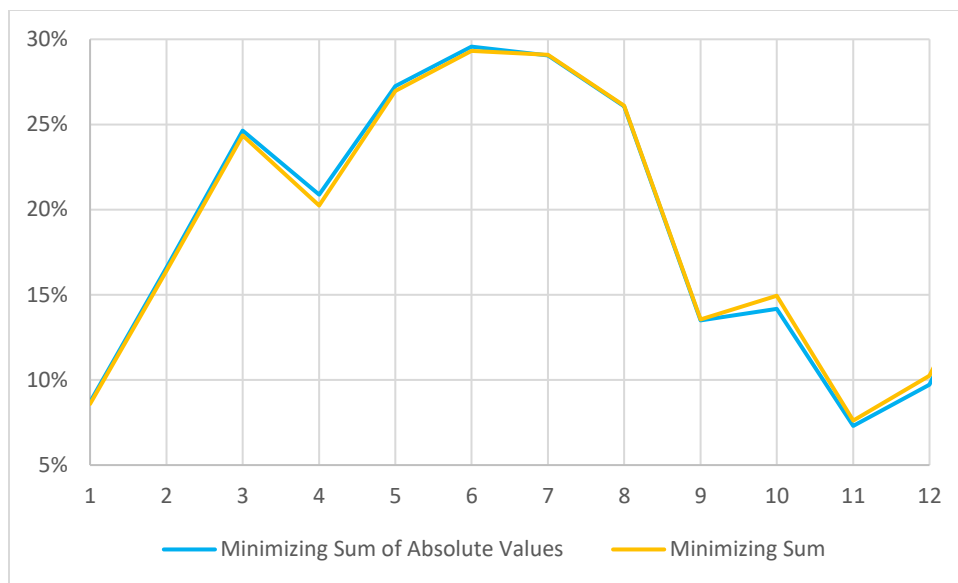
Figure 19: Weighted Capacity Factors: Absolute Value vs. Sum
