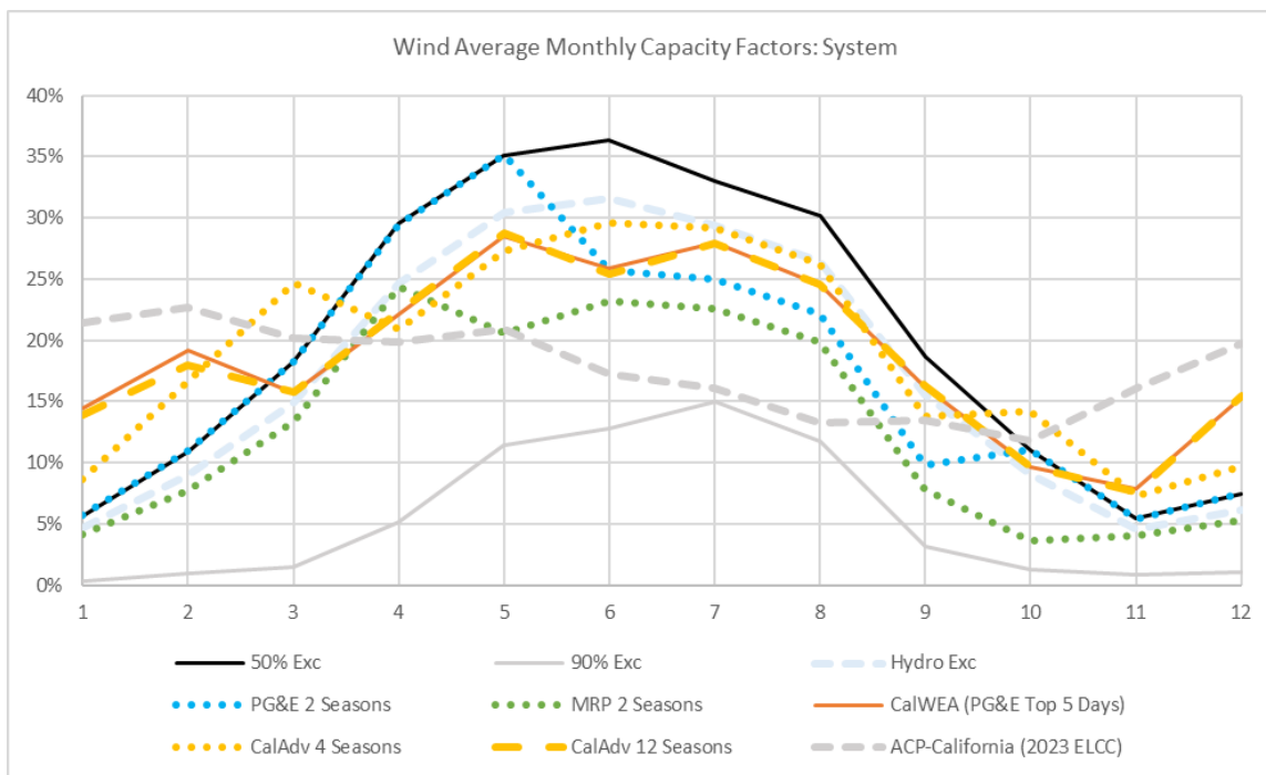
Figure 41: Wind Average Monthly Capacity Factors: System
