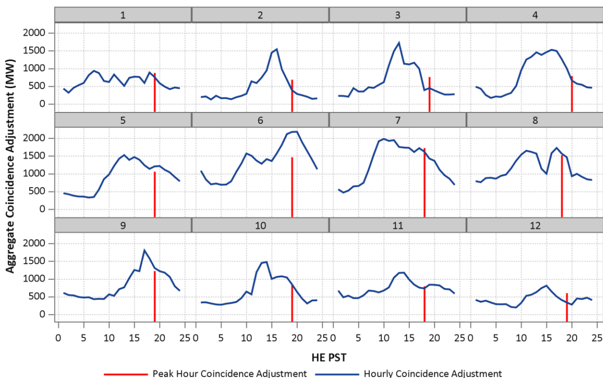
Figure 1: Comparison of Peak-Hour and Hourly Aggregate Coincidence Adjustments by Month
