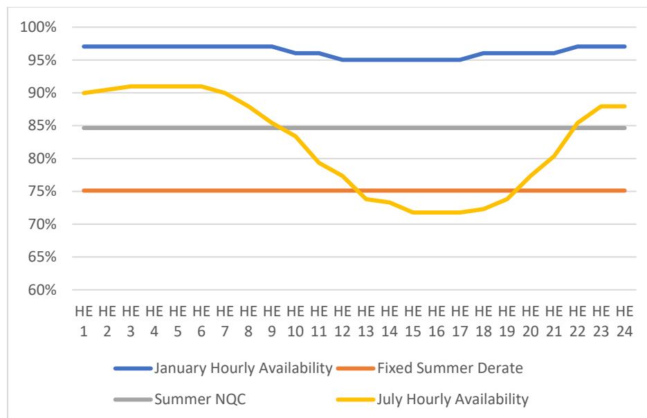
Figure 51: Hourly Pattern of Facilities' Ambient Derates
