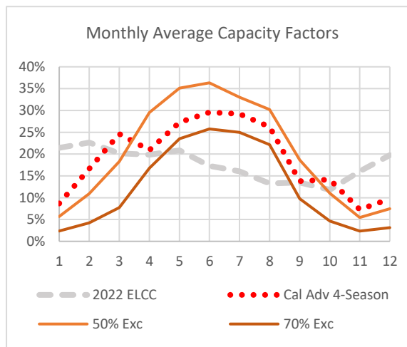
Figure 18: Monthly Average Capacity Factors
