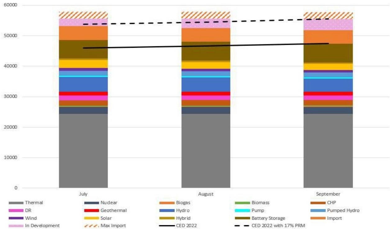
Figure 19. Stack Analysis of Current Resource Adequacy Framework for July – September 2024.
