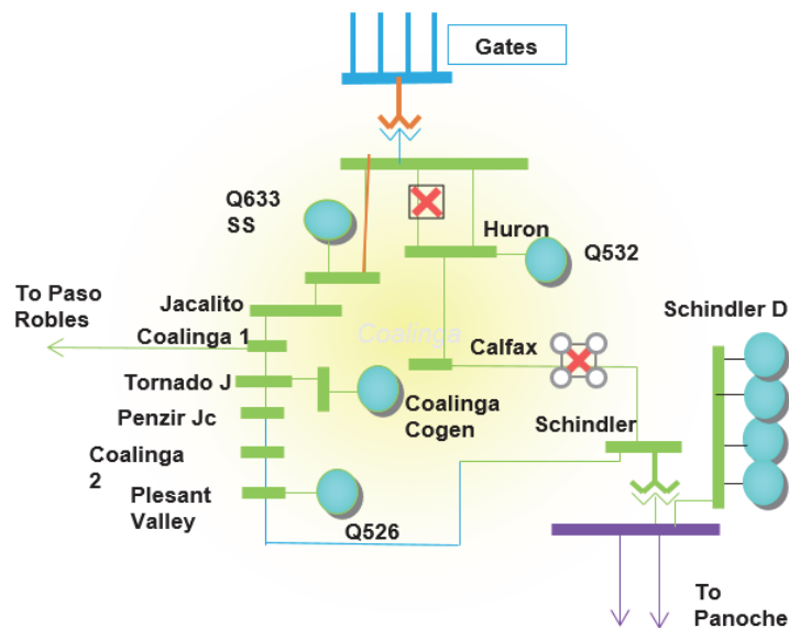
Figure 3.3-50 Coalinga LCR Sub-area
