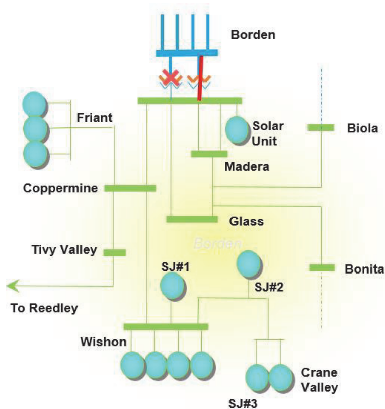
Figure 3.3-53 Borden LCR Sub-area
