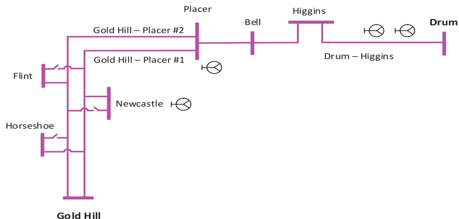
Figure 3.3-14 Placer LCR Sub-area
