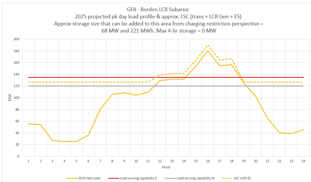
Figure 3.3-54 Borden LCR Sub-area 2025 Peak Day Forecast Profiles
