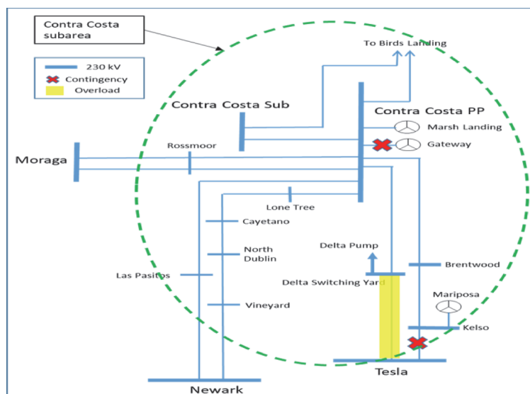
Figure 3.3-43 Contra Costa LCR Sub-area
