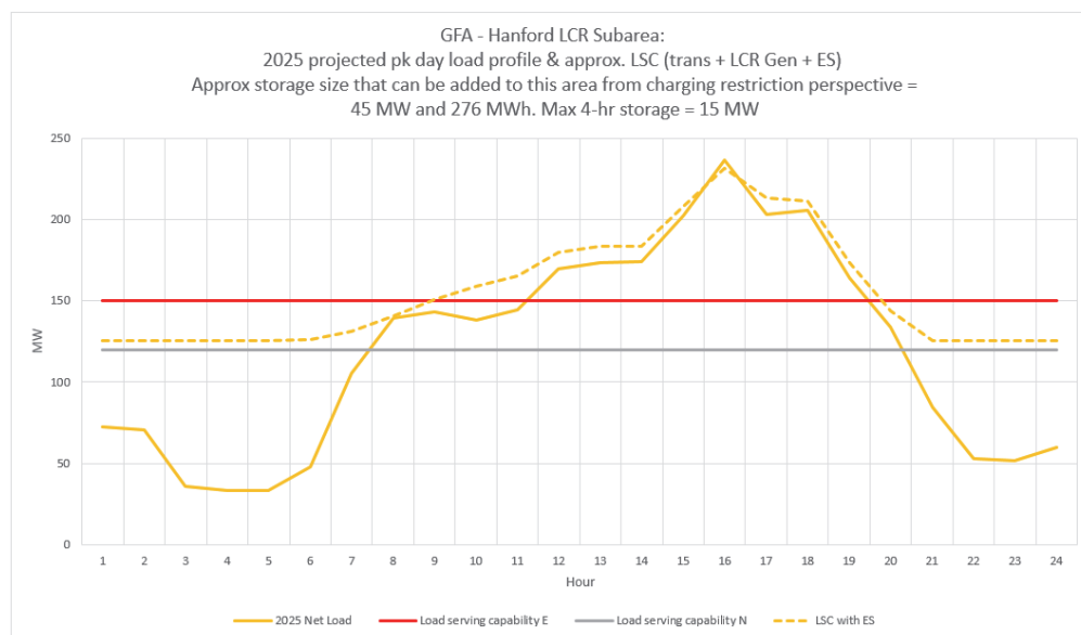
Figure 3.3-48 Hanford LCR Sub-area 2025 Peak Day Forecast Profiles
