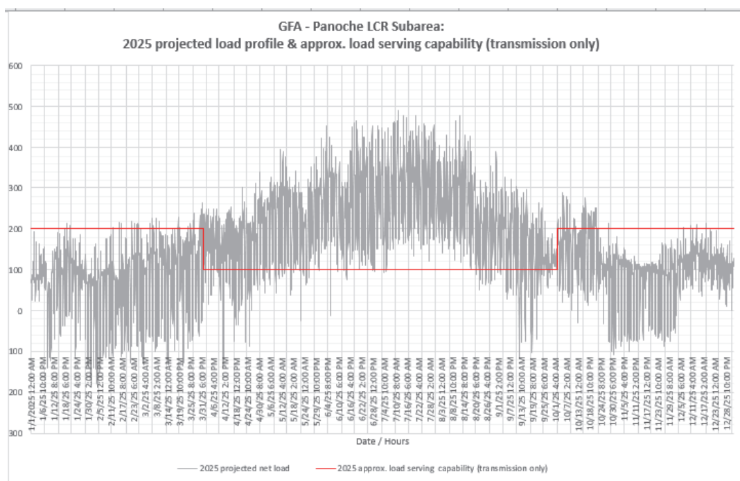
Figure 3.3-61 Panoche LCR Sub-area 2025 Forecast Hourly Profiles
