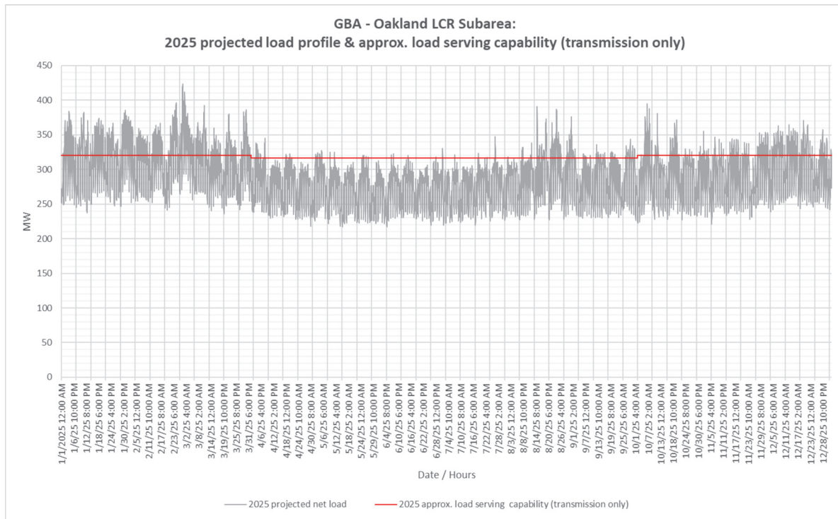
Figure 3.3-41 Oakland LCR Sub-area 2025 Forecast Hourly Profiles
