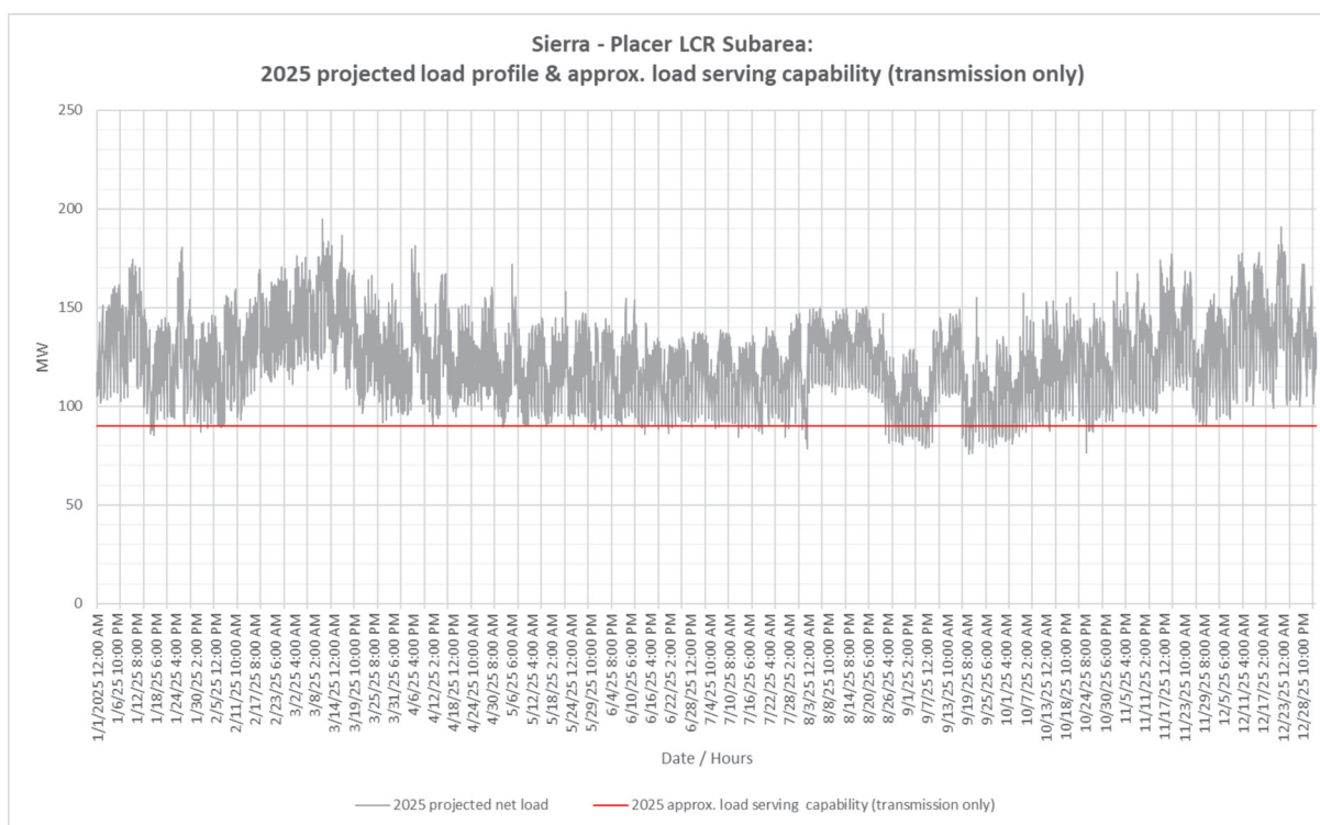
Figure 3.3-16 Placer LCR Sub-area 2025 Forecast Hourly Profiles
