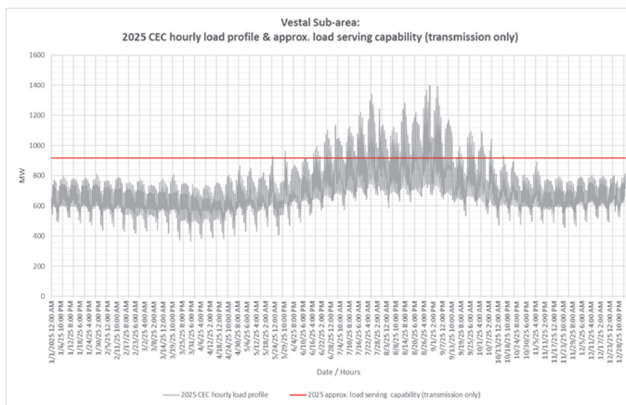
Figure 3.3-78 Vestal LCR Sub-area 2025 Annual Load Profile with Estimated Transmission Only Load Serving Capability
