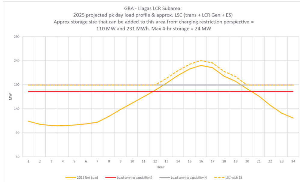
Figure 3.3-34 Llagas LCR Sub-area 2025 Forecast Hourly Profiles
