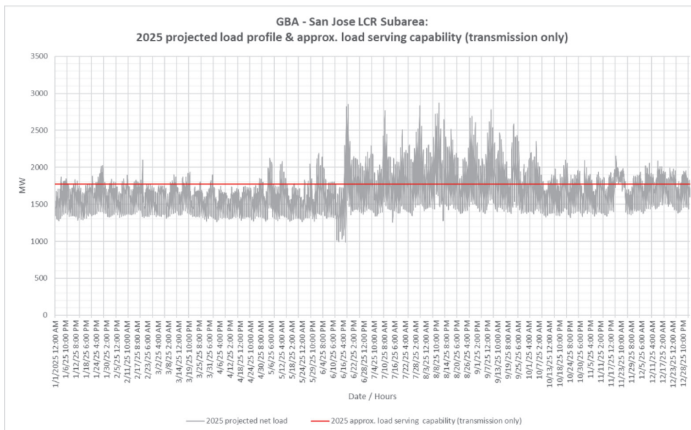
Figure 3.3-36 San Jose LCR Sub-area 2025 Forecast Hourly Profiles
