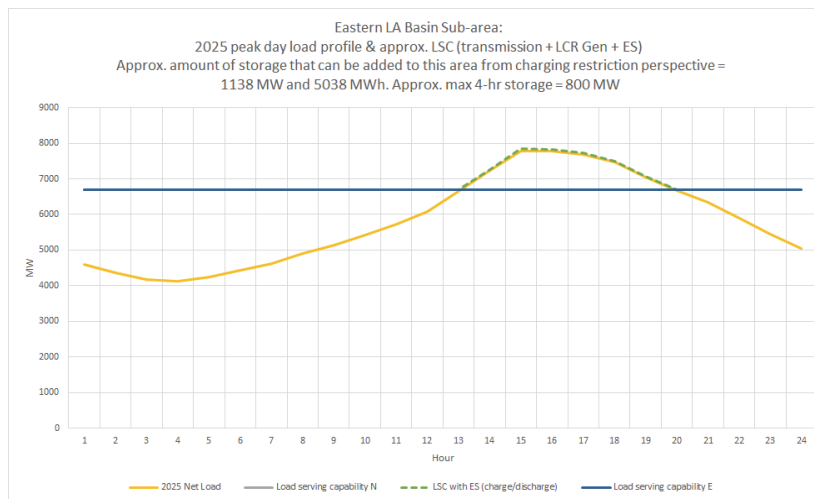
Figure 3.3-91 Eastern LA Basin LCR Sub-area 2025 Load Shape and Estimated Maximum Energy Storage Capacity and Energy Based on Charging Capability Under Critical Contingency
