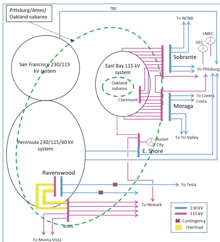
Figure 3.3-42 Ames-Pittsburg-Oakland LCR Sub-area
