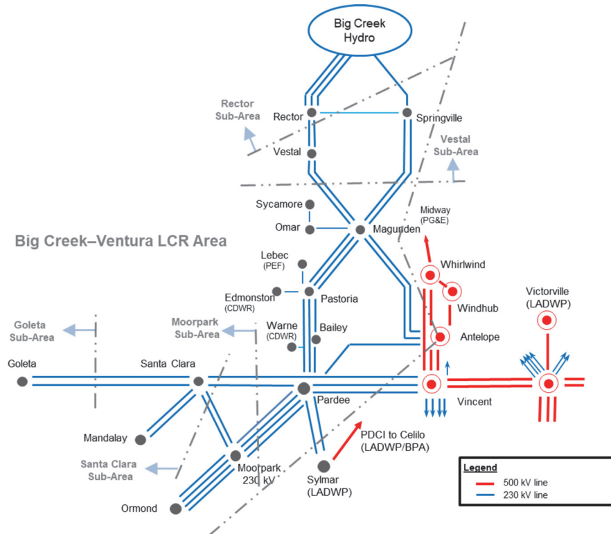
Figure 3.3-76 Big Creek/Ventura LCR Area
