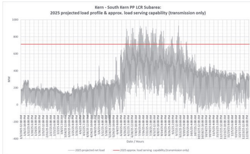
Figure 3.3-75 South Kern PP LCR Sub-area 2025 Forecast Hourly Profiles
