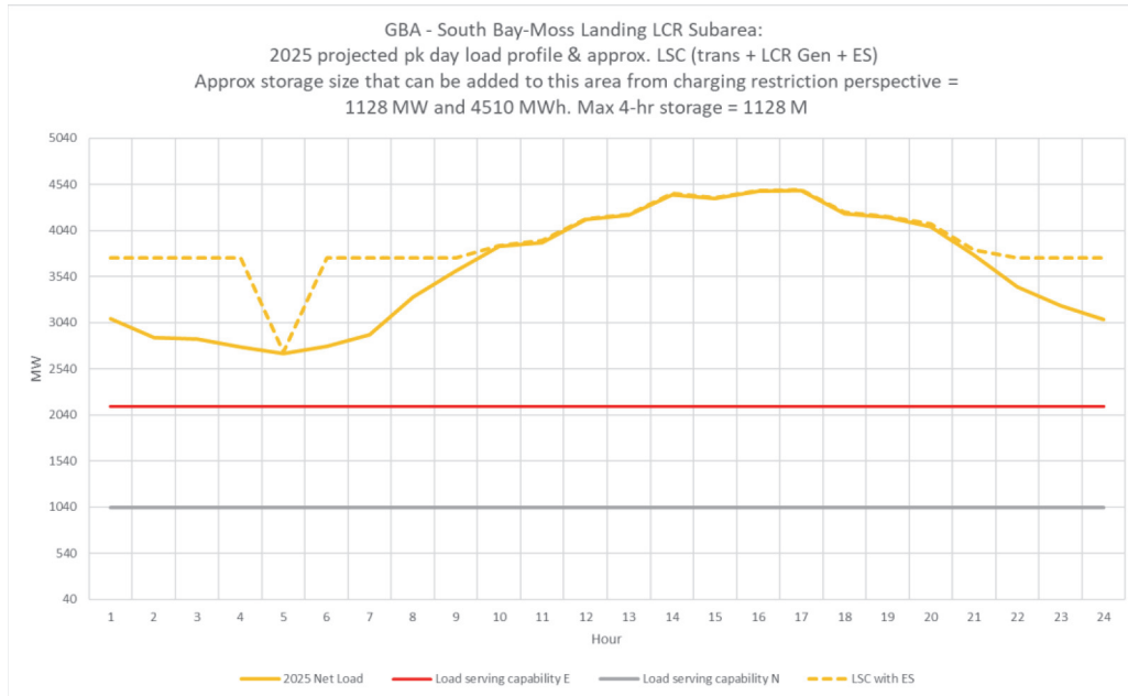
Figure 3.3-38 South Bay-Moss Landing LCR Sub-area 2025 Forecast Hourly Profiles
