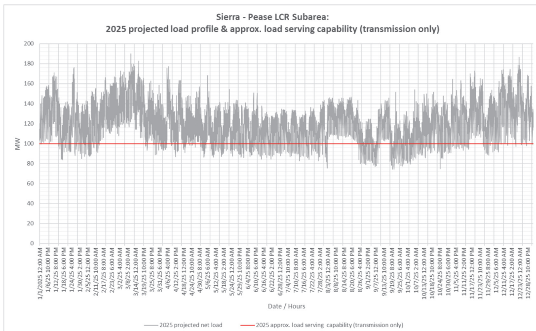
Figure 3.3-19 Pease LCR Sub-area 2025 Forecast Hourly Profiles
