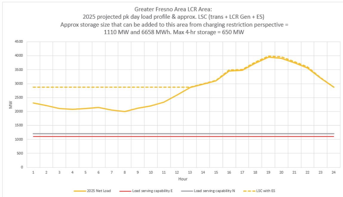
Figure 3.3-67 Fresno LCR area 2025 Peak Day Forecast Profiles
