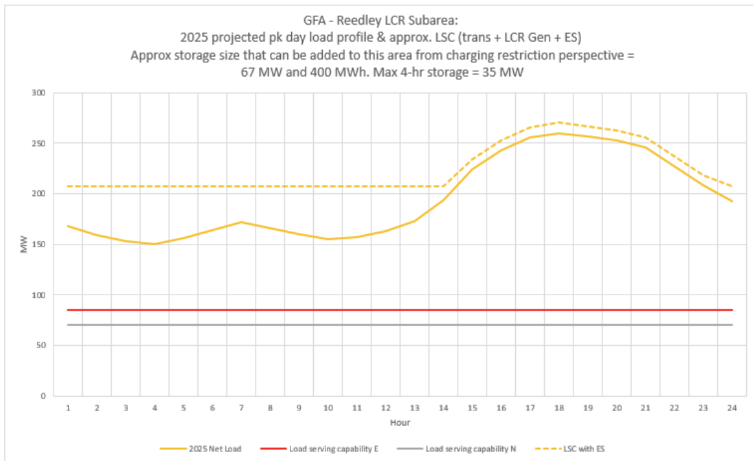
Figure 3.3-57 Reedley LCR Sub-area 2025 Peak Day Forecast Profiles
