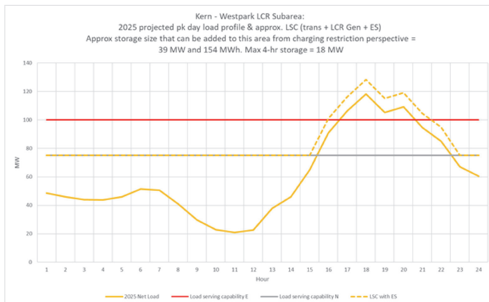
Figure 3.3-70 Westpark LCR Sub-area 2025 Peak Day Forecast Profiles
