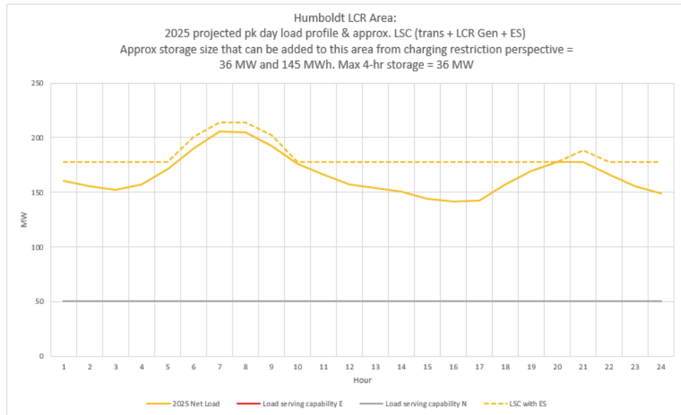
Figure 3.3-3 Humboldt 2025 Forecast Hourly Profile
