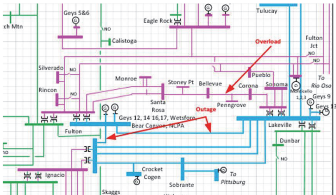
Figure 3.3-10 Fulton LCR Sub-area
