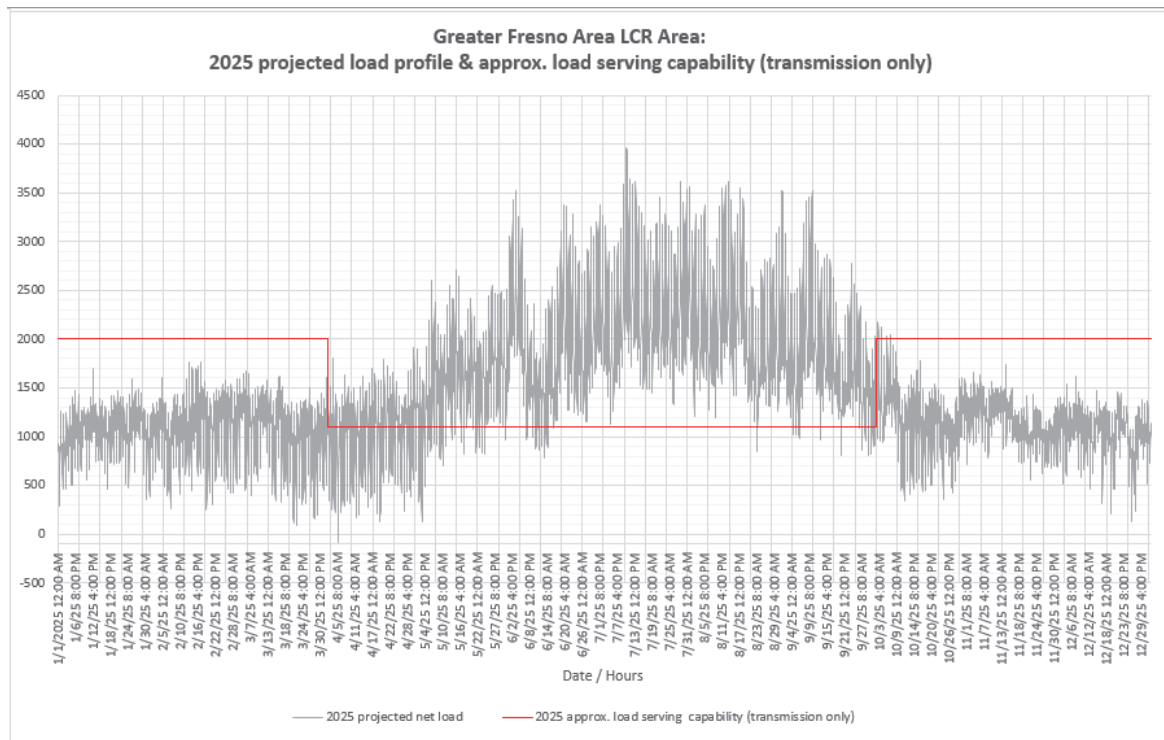
Figure 3.3-68 Fresno LCR area 2025 Forecast Hourly Profiles
