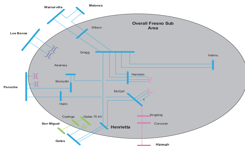
Figure 3.3-46 Fresno LCR Area
