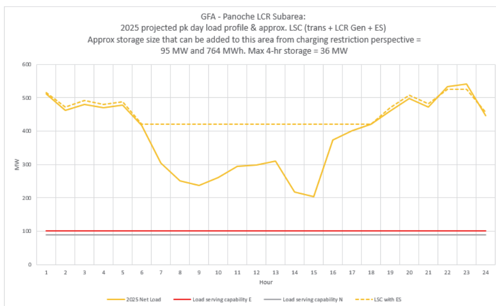
Figure 3.3-60 Panoche LCR Sub-area 2025 Peak Day Forecast Profiles
