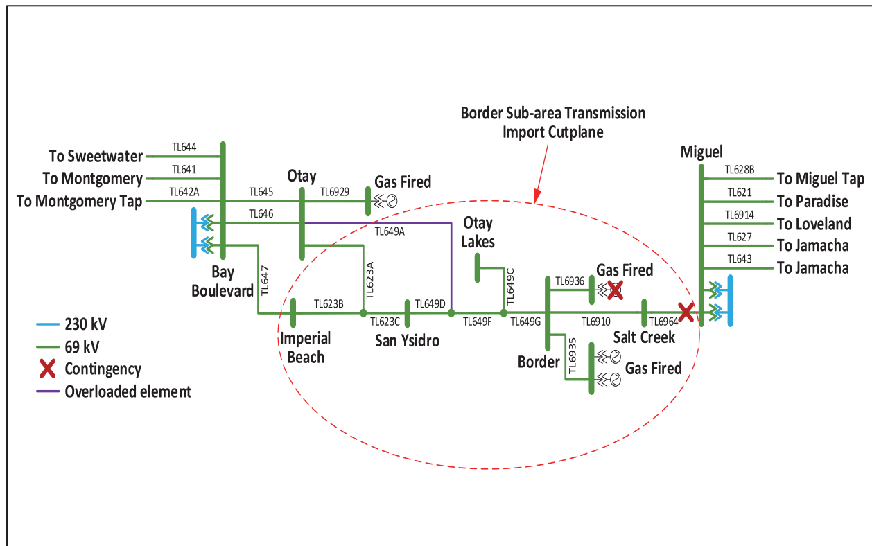
Figure 3.3-96 Border LCR Sub-area
