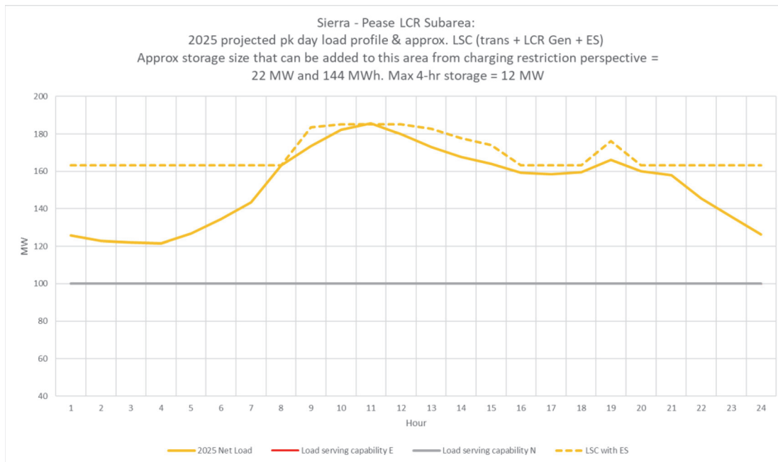
Figure 3.3-19 Pease LCR Sub-area 2025 Forecast Hourly Profiles
