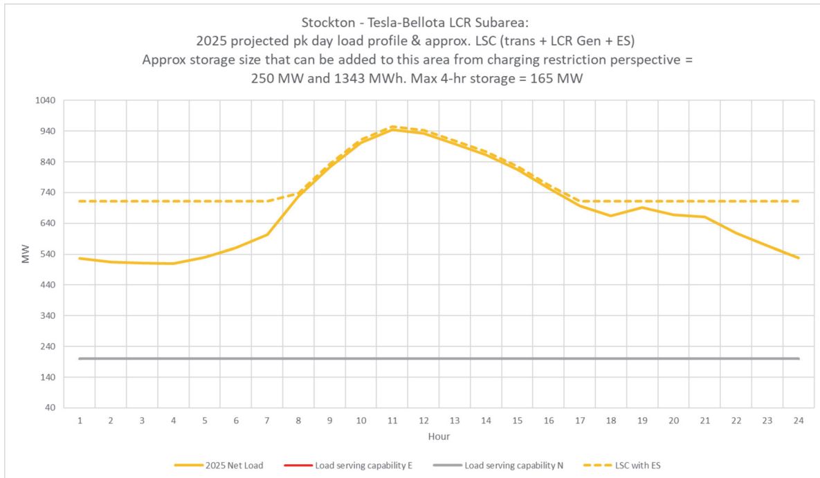
Figure 3.3-30 Tesla-Bellota LCR Sub-area 2025 Forecast Hourly Profiles
