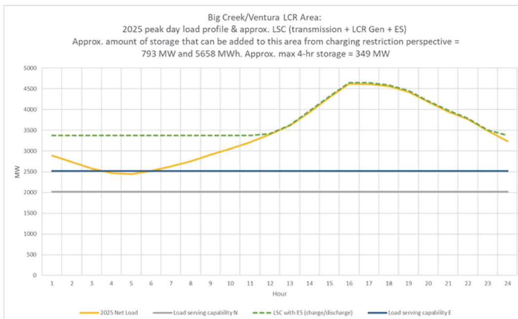
Figure 3.3-84 Big Creek/Ventura LCR area 2025 Load Shape and Estimated Maximum Energy Storage Capacity and Energy Based on Charging Capability Under Critical Contingency
