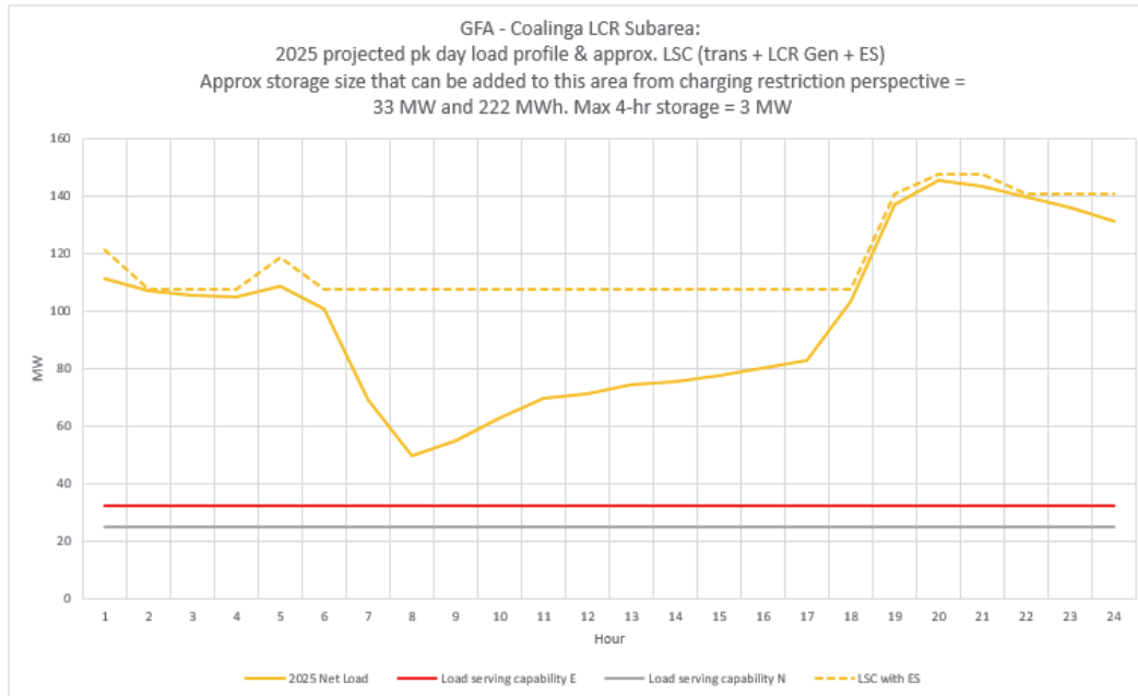
Figure 3.3-52 Coalinga LCR Sub-area 2025 Forecast Hourly Profiles
