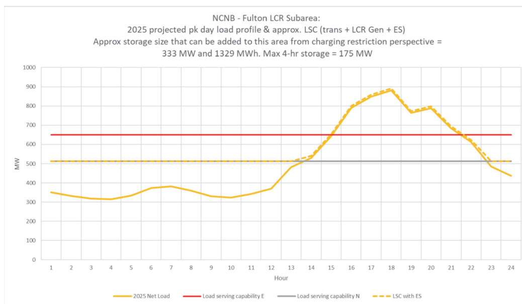
Figure 3.3-11 Fulton LCR Sub-area 2025 Peak Day Forecast Profiles
