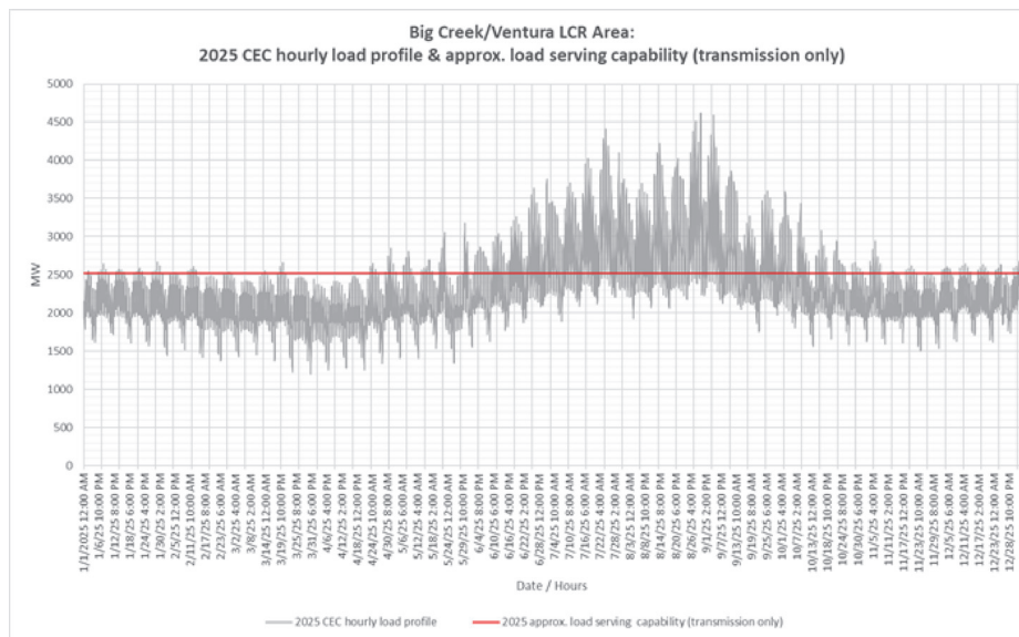
Figure 3.3-83 Big Creek/Ventura LCR area 2025 Annual Load Profile with Estimated Transmission Only Load Serving Capability
