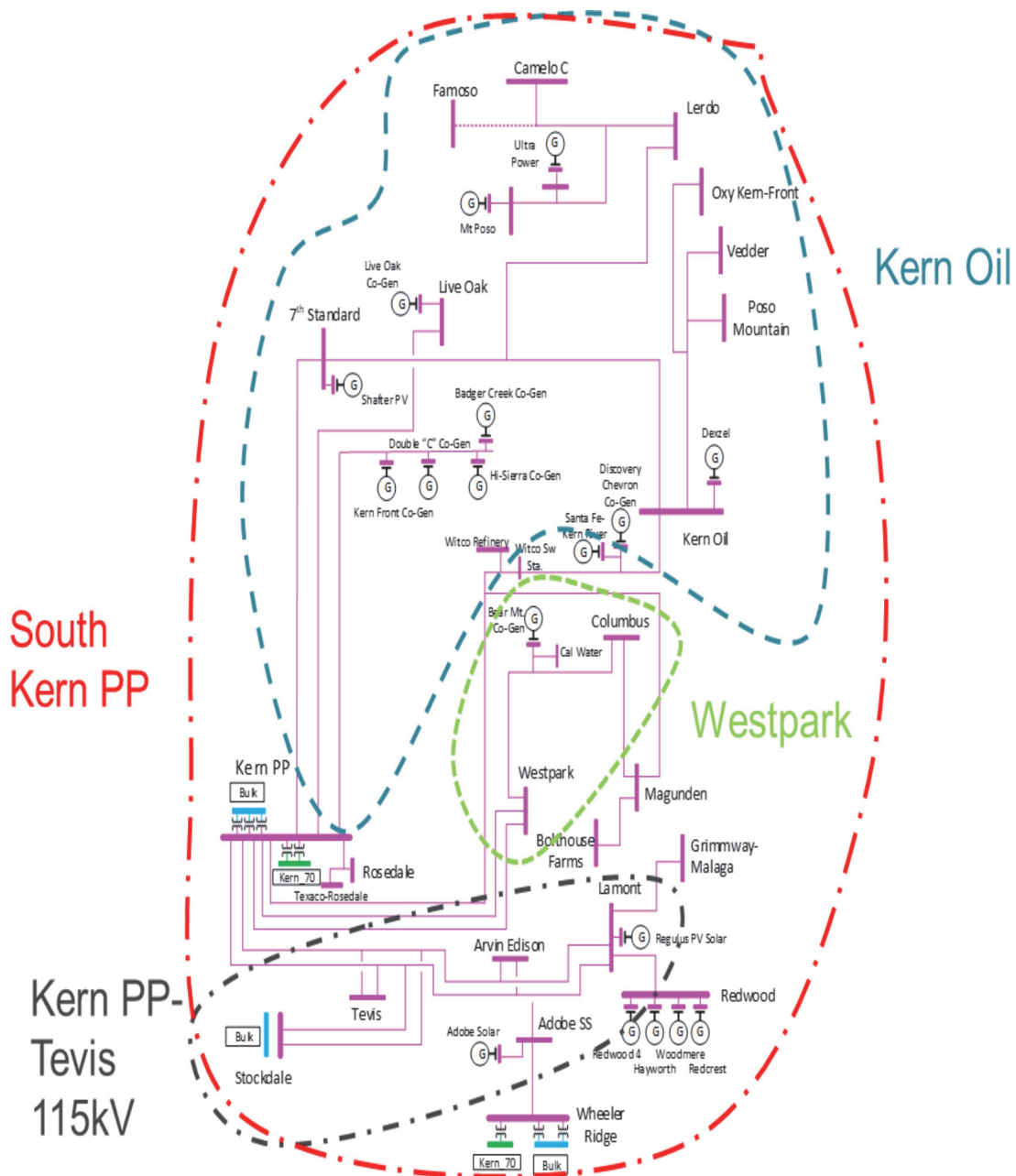
Figure 3.3-69 Kern LCR Sub-area
