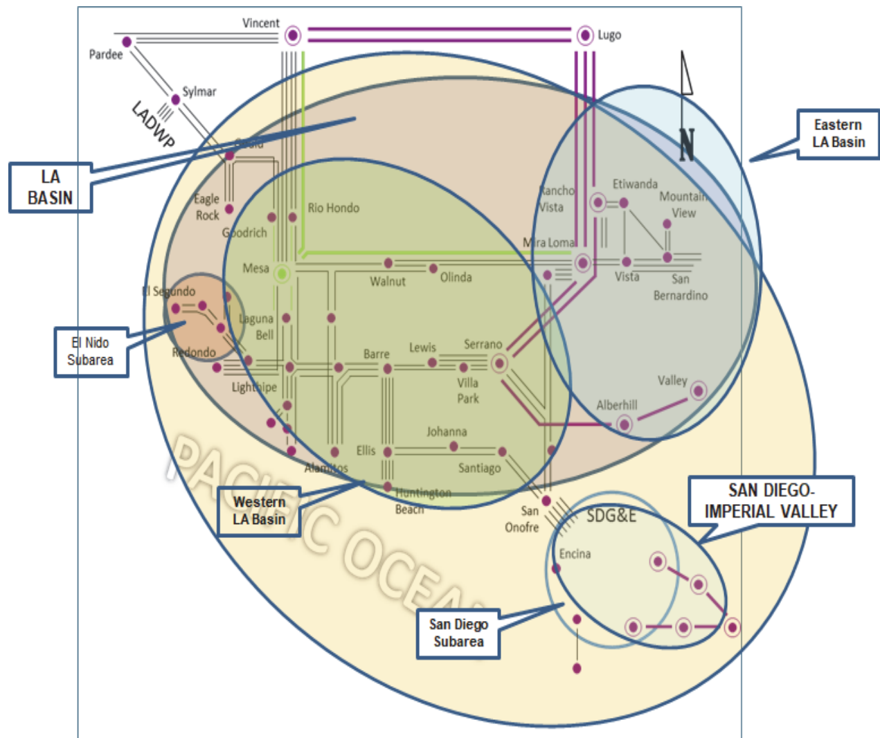
Figure 3.3-92 San Diego-Imperial Valley LCR Area
