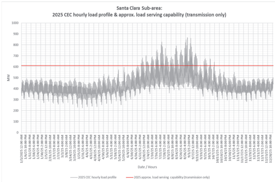
Figure 3.3-81 Santa Clara LCR Sub-area 2025 Annual Load Profile with Estimated Transmission Only Load Serving Capability
