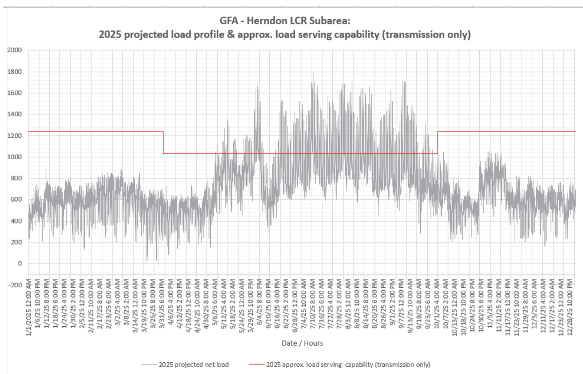
Figure 3.3-65 Herndon LCR Sub-area 2025 Forecast Hourly Profiles
