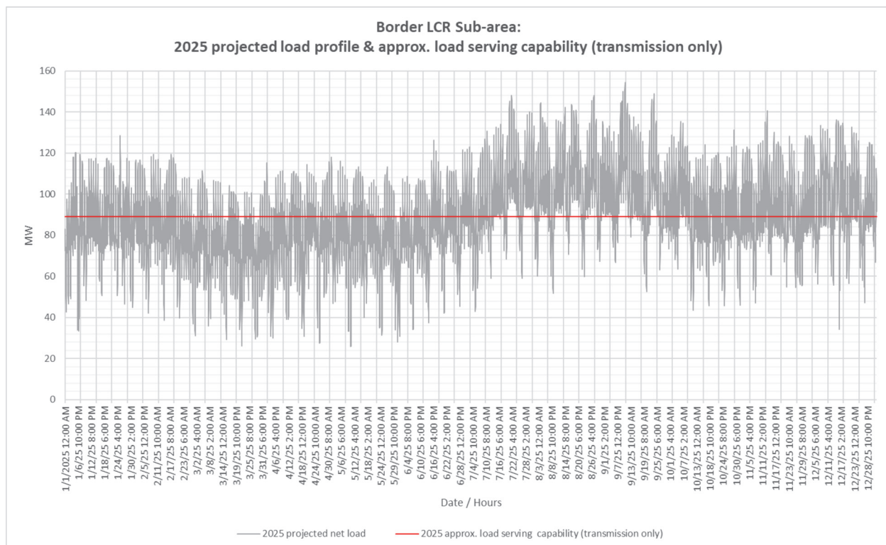
Figure 3.3-98 Border LCR Sub-area 2025 Peak Day Forecast Profiles
