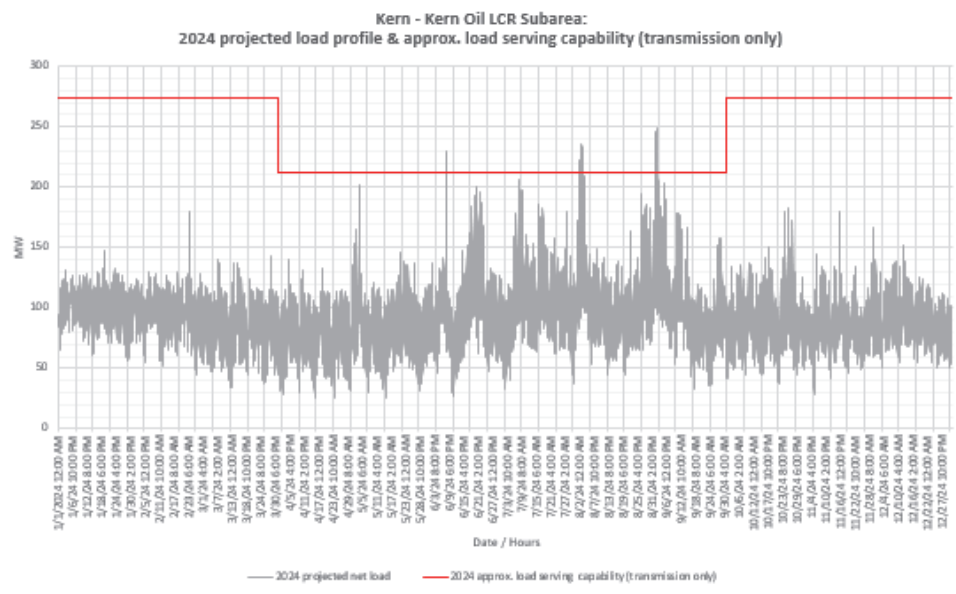
Figure 3.3-73 Kern Oil LCR Sub-area 2025 Forecast Hourly Profiles
