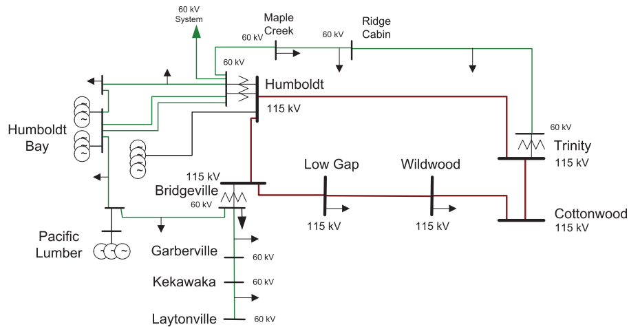
Figure 3.3-1 Humboldt LCR Area
