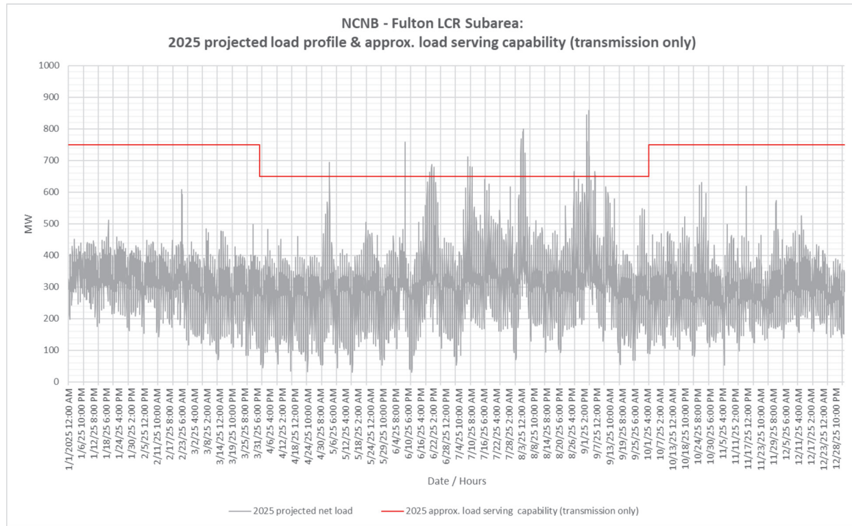
Figure 3.3-12 Fulton LCR Sub-area 2025 Forecast Hourly Profiles
