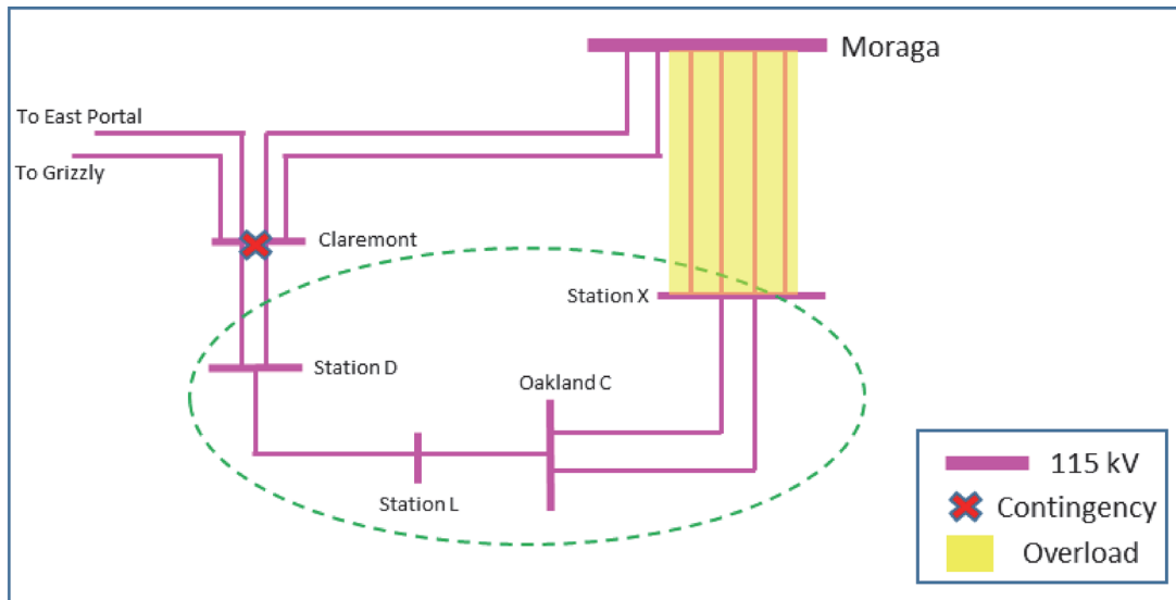
Figure 3.3-39 Oakland LCR Sub-area
