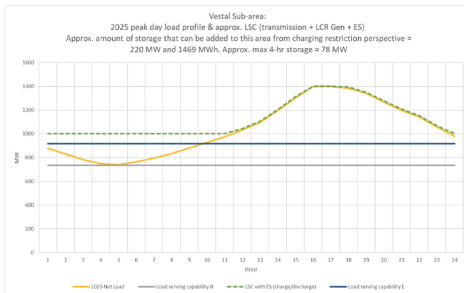
Figure 3.3-79 Vestal LCR Sub-area 2025 Load Shape and Estimated Maximum Energy Storage Capacity and Energy Based on Charging Capability Under Critical Contingency
