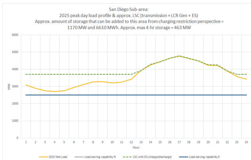
Figure 3.3-100 San Diego LCR Sub-area 2025 Load Shape and Estimated Maximum Energy Storage Capacity and Energy Based on Charging Capability Under Critical Contingency
