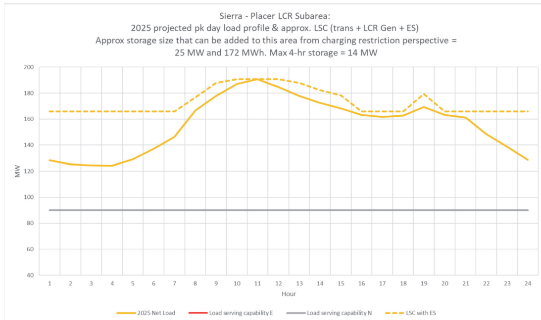
Figure 3.3-15 Placer LCR Sub-area 2025 Peak Day Forecast Profiles
