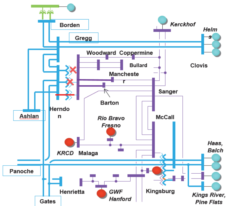
Figure 3.3-63 Herndon LCR Sub-area
