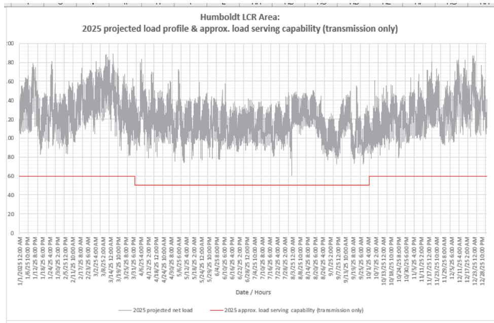
Figure 3.3-3 Humboldt 2025 Forecast Hourly Profile
