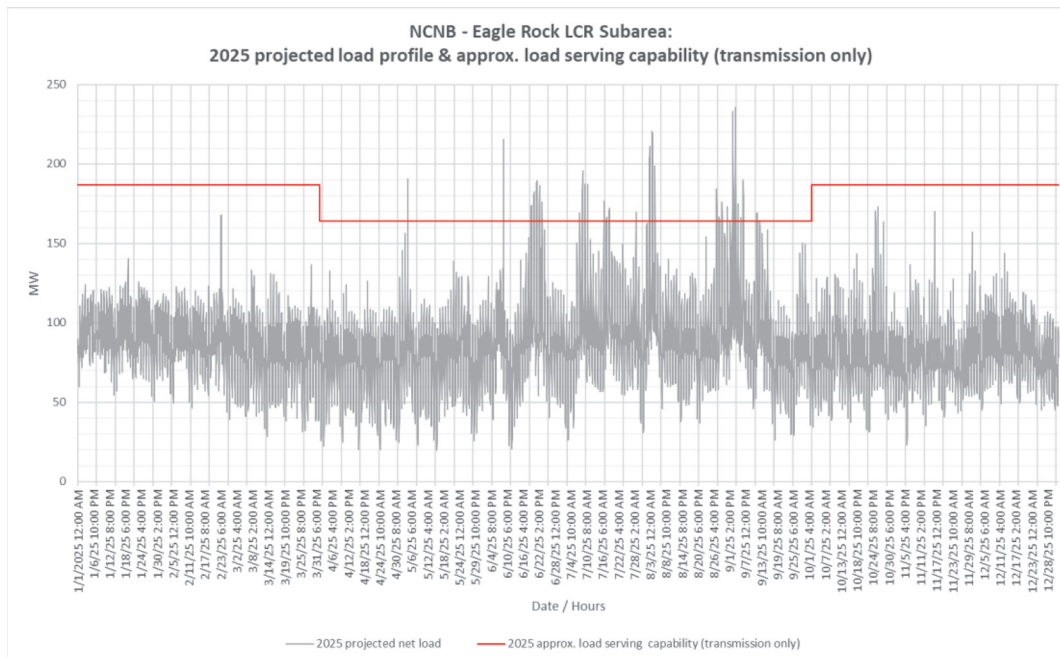
Figure 3.3-9 Eagle Rock LCR Sub-area 2025 Forecast Hourly Profiles
