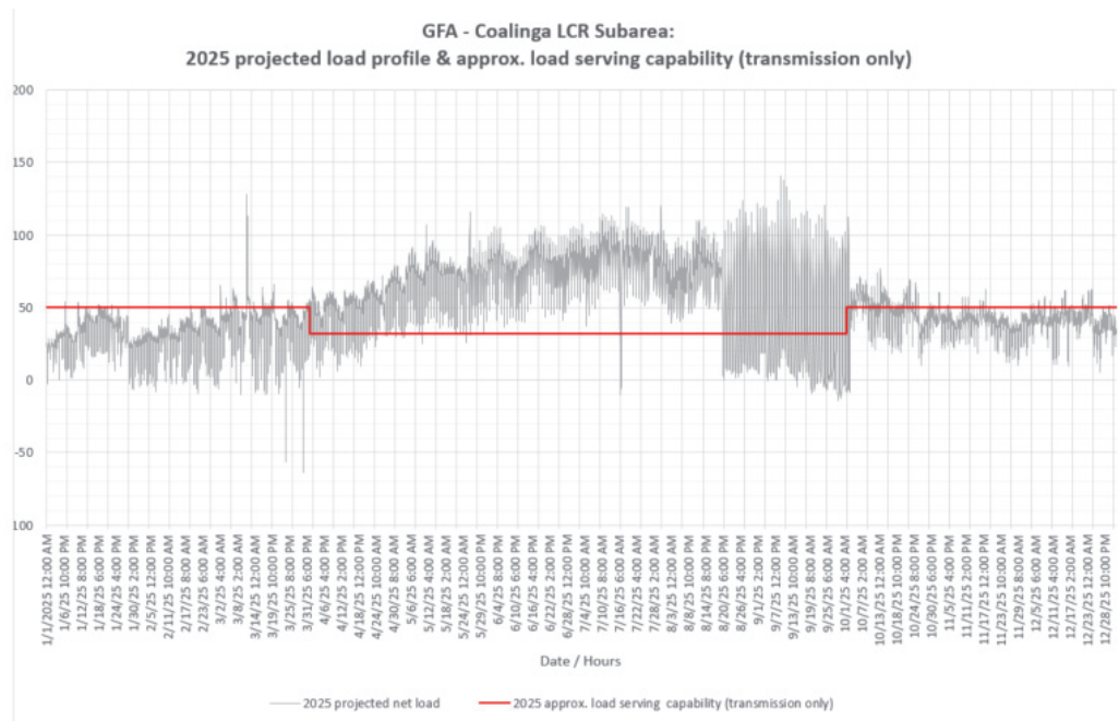
Figure 3.3-52 Coalinga LCR Sub-area 2025 Forecast Hourly Profiles
