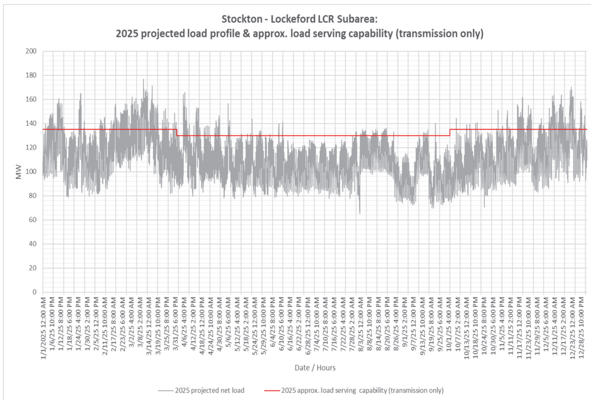
Figure 3.3-26 Lockeford LCR Sub-area 2025 Forecast Hourly Profiles
