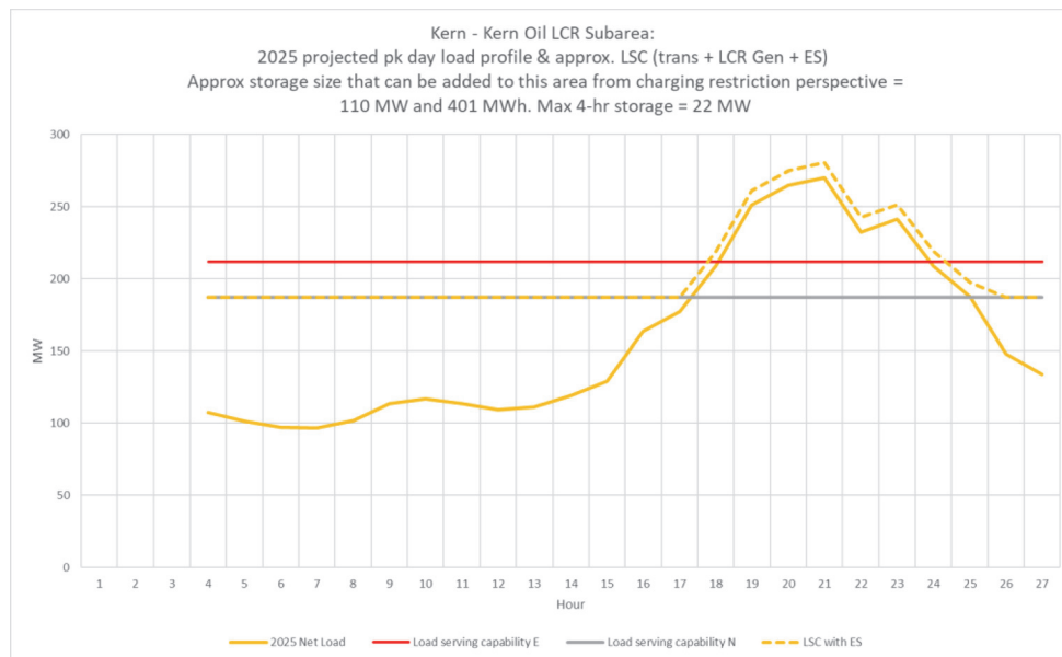
Figure 3.3-72 Kern Oil LCR Sub-area 2025 Peak Day Forecast Profiles
