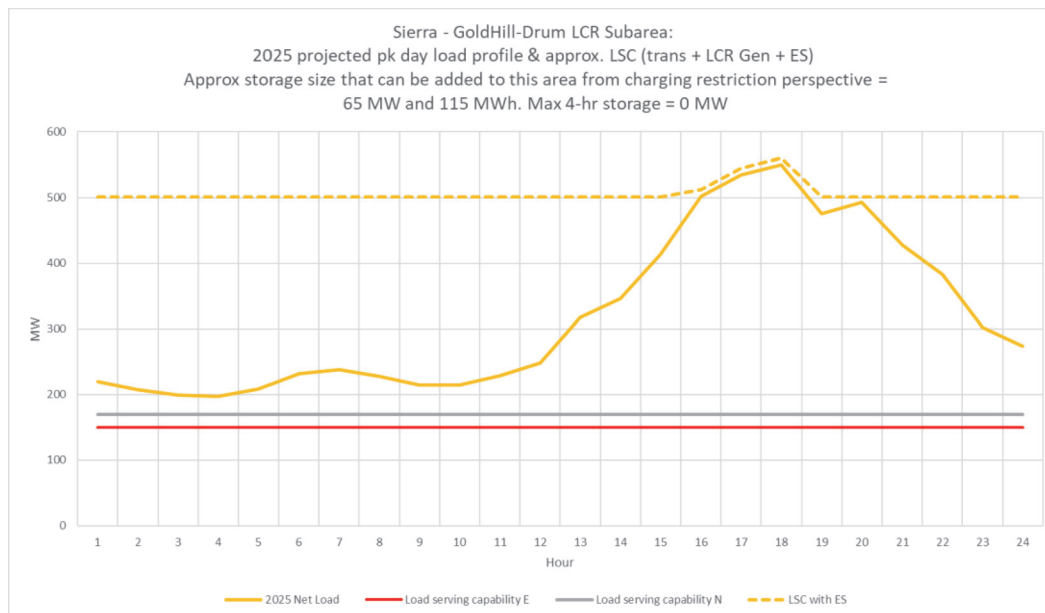
Figure 3.3-21 Gold Hill-Drum LCR Sub-area 2025 Peak Day Forecast Profiles
