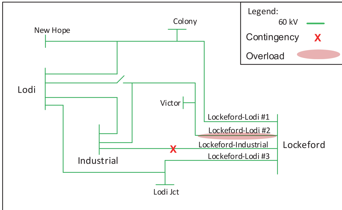
Figure 3.3-24 Lockeford LCR Sub-area
