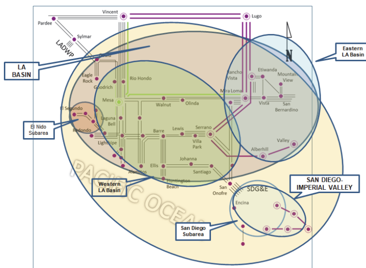
Figure 3.3-85 LA Basin LCR Area
