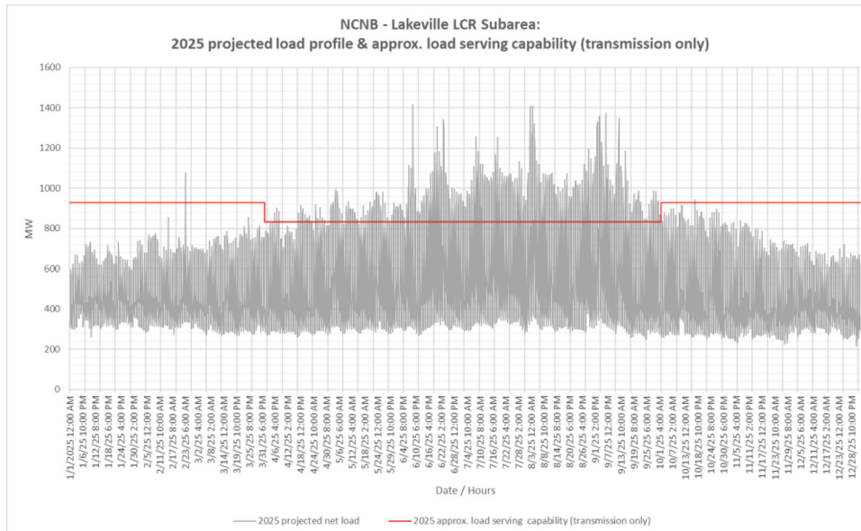
Figure 3.3-6 North Coast and North Bay 2025 Forecast Hourly Profile
