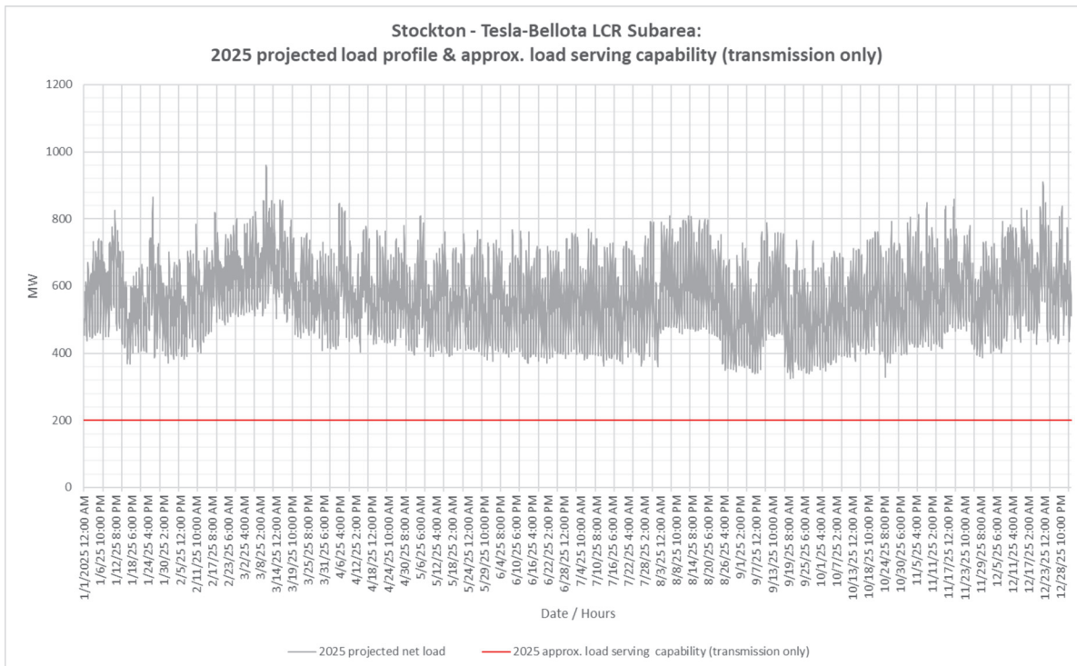
Figure 3.3-30 Tesla-Bellota LCR Sub-area 2025 Forecast Hourly Profiles
