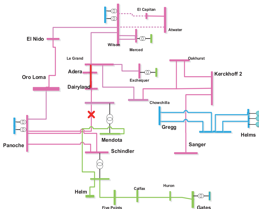
Figure 3.3-59 Panoche LCR Sub-area
