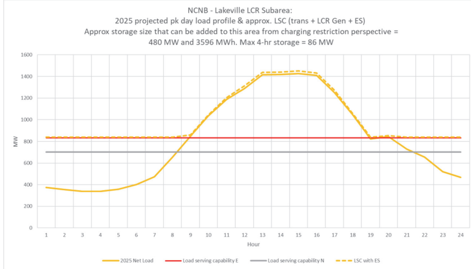
Figure 3.3-6 North Coast and North Bay 2025 Forecast Hourly Profile
