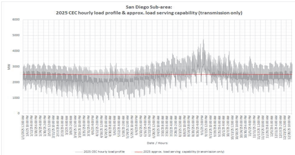
Figure 3.3-99 San Diego LCR Sub-area 2025 Annual Load Profile with Estimated Transmission Load Serving Capability Only
