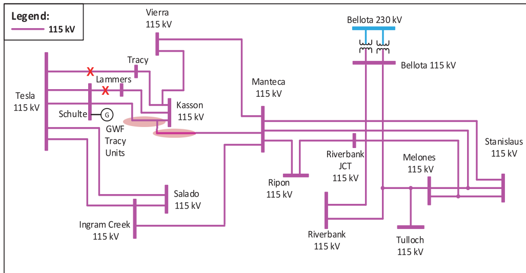
Figure 3.3-28 Tesla-Bellota LCR Sub-area
