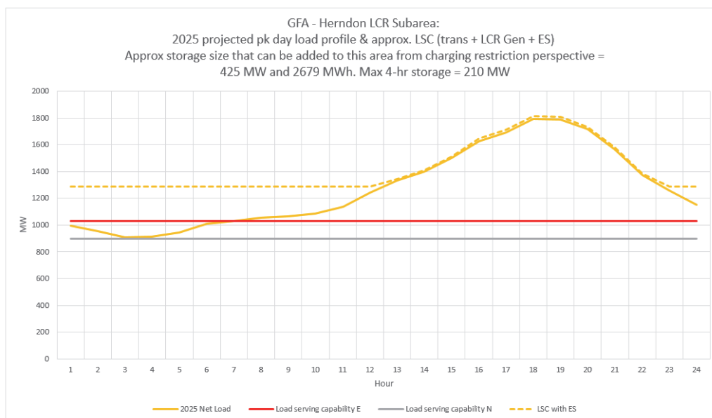
Figure 3.3-64 Herndon LCR Sub-area 2025 Peak Day Forecast Profiles
