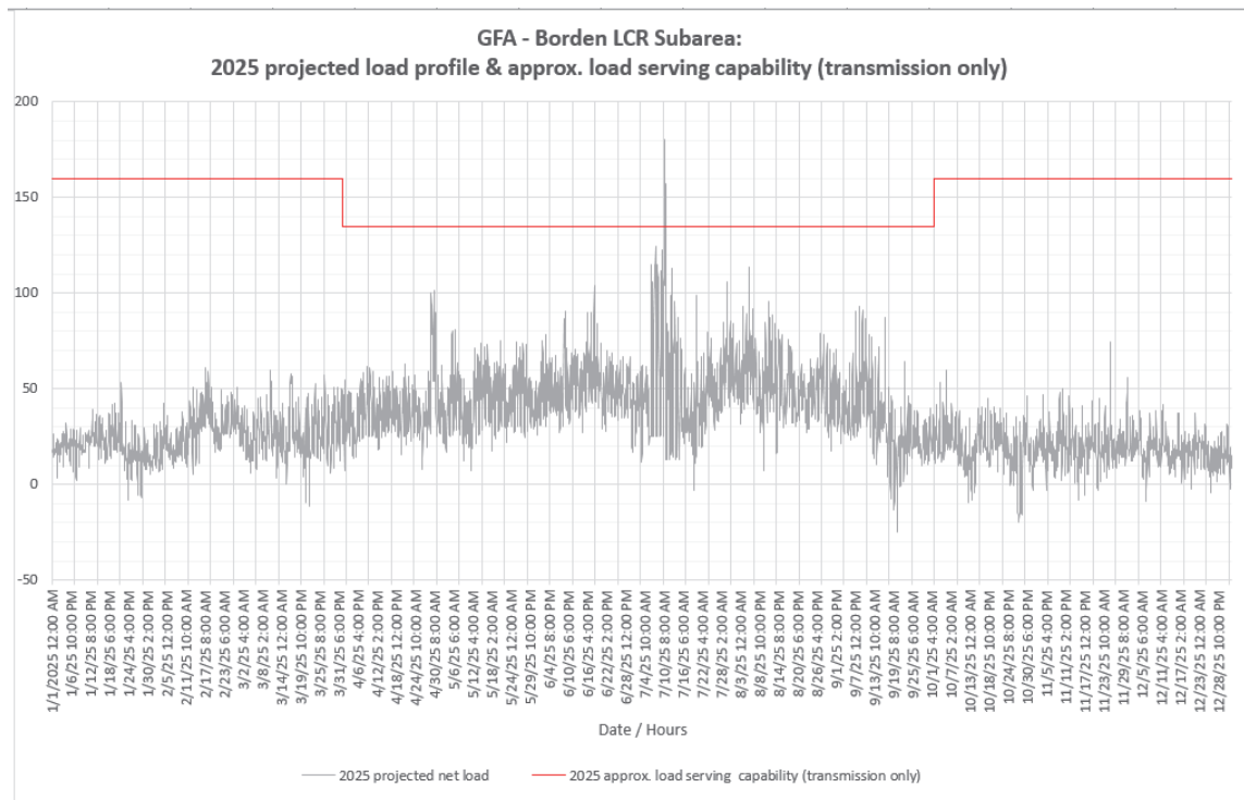
Figure 3.3-55 Borden LCR Sub-area 2025 Forecast Hourly Profiles
