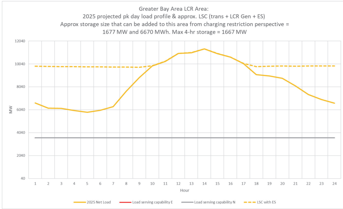
Figure 3.3-45 Bay Area LCR Area 2025 Forecast Hourly Profiles
