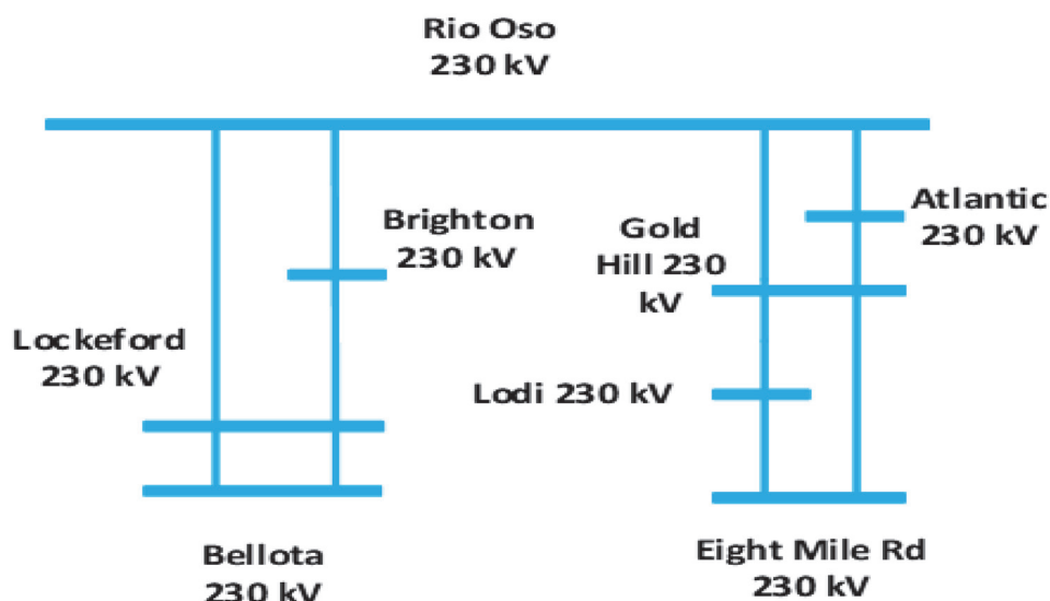
Figure 3.3-23 South of Rio Oso LCR Sub-area
