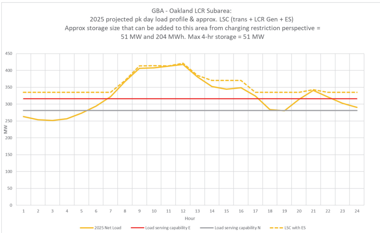
Figure 3.3-40 Oakland LCR Sub-area 2025 Peak Day Forecast Profiles
