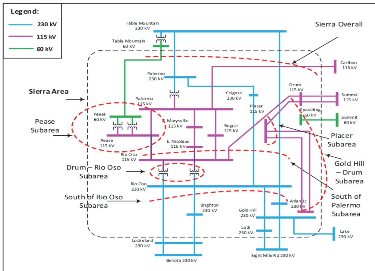
Figure 3.3-13 Sierra LCR Area
