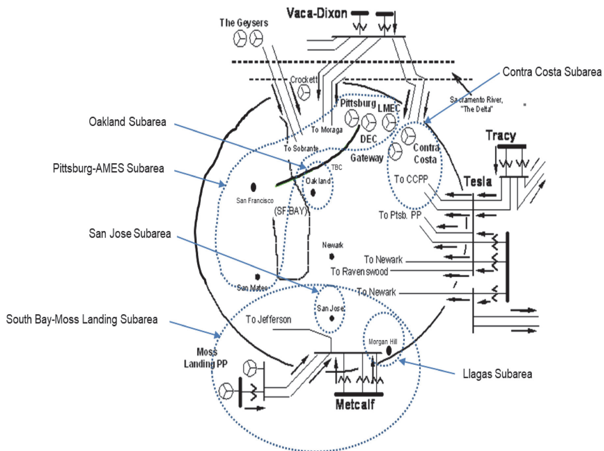
Figure 3.3-31 Greater Bay LCR Area
