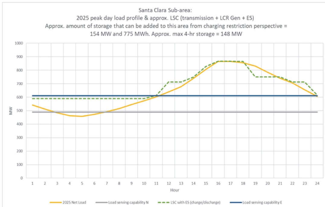
Figure 3.3-82 Santa Clara LCR Sub-area 2025 Load Shape and Estimated Maximum Energy Storage Capacity and Energy Based on Charging Capability Under Critical Contingency
