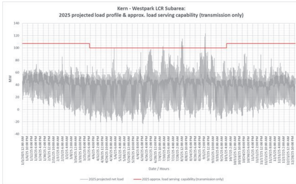
Figure 3.3-71 Westpark LCR Sub-area 2025 Forecast Hourly Profiles
