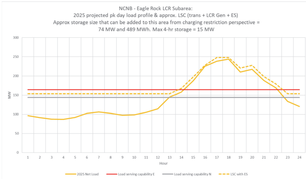
Figure 3.3-9 Eagle Rock LCR Sub-area 2025 Forecast Hourly Profiles
