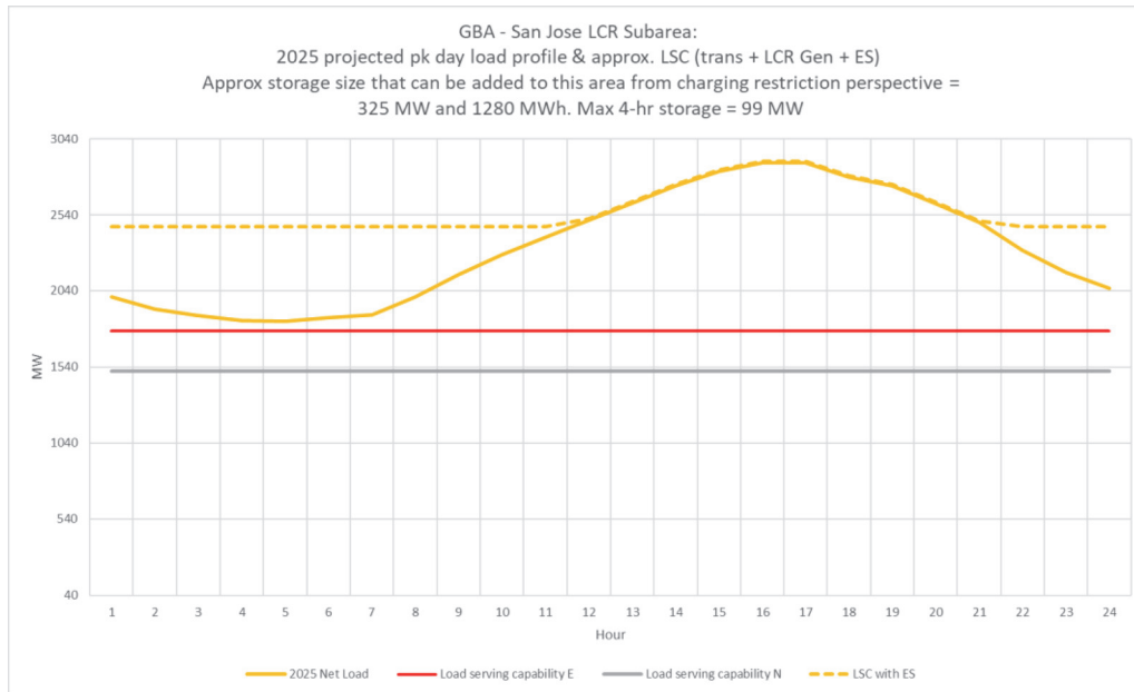
Figure 3.3-36 San Jose LCR Sub-area 2025 Forecast Hourly Profiles
