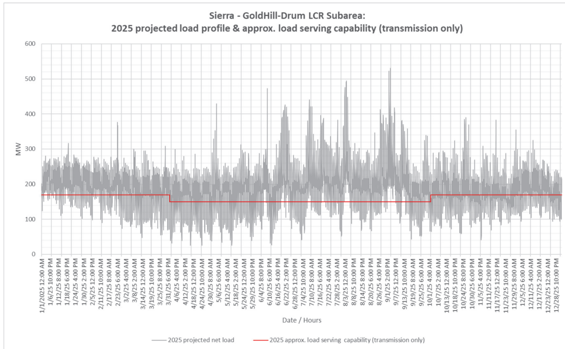
Figure 3.3-22 Gold Hill-Drum LCR Sub-area 2025 Forecast Hourly Profiles
