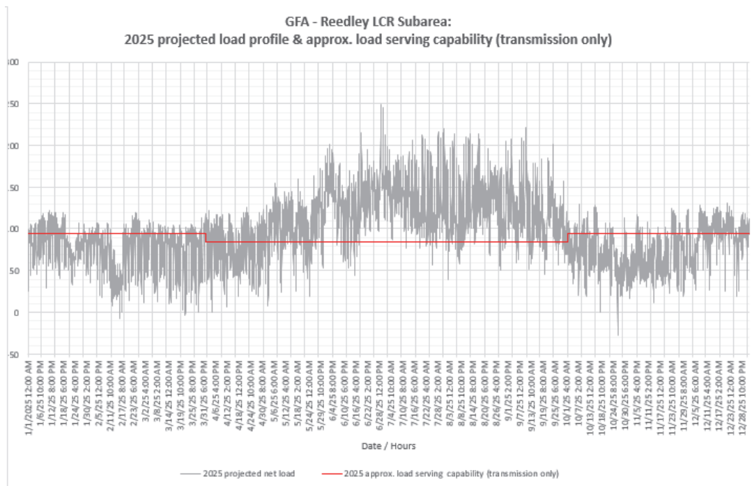
Figure 3.3-58 Reedley LCR Sub-area 2025 Forecast Hourly Profiles
