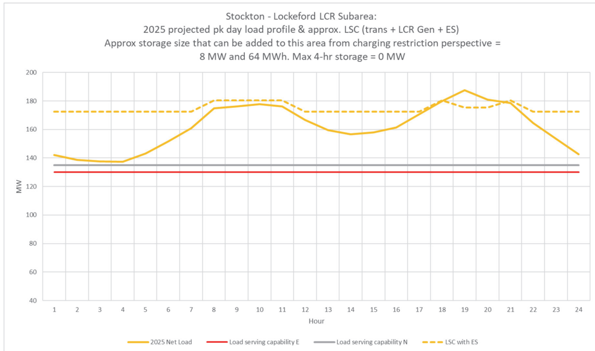
Figure 3.3-26 Lockeford LCR Sub-area 2025 Forecast Hourly Profiles
