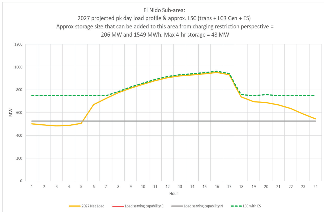
Figure 3.3-86 El Nido LCR Sub-area 2027 Load Shape and Estimated Maximum Energy Storage Capacity and Energy Based on Charging Capability Under Critical Contingency
