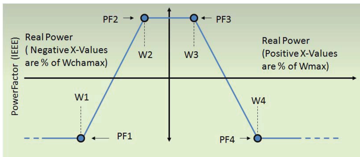
Figure 26: Example Watt – Power Factor Configuration
