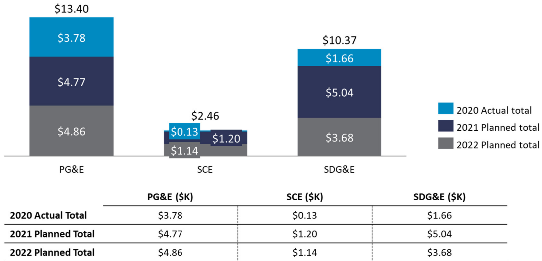
Actual and projected spend ($K) per HFTD overhead circuit mile
