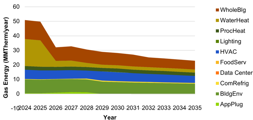
Figure 4-11. C&S Gas Savings (Including Interactive Effects)
