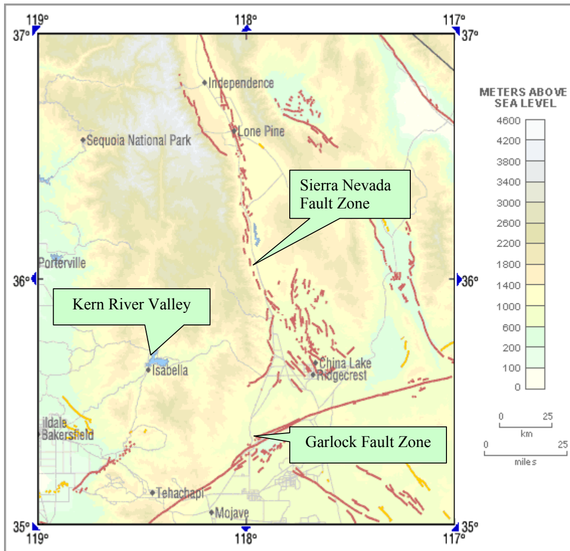
Major Fault Lines near the Kern River Valley District
