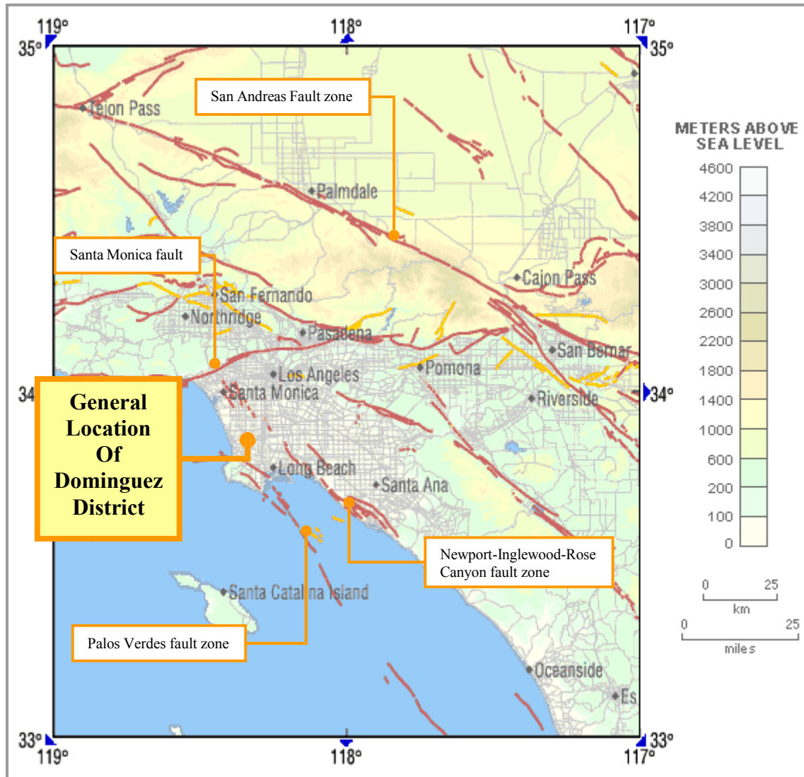
Major Fault Lines near the Rancho Dominguez District
