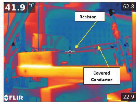
11:15 AM Energized –Test Subject Temp.: 41.9°C
