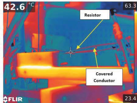
11:13 AM De-Energized –Conductor Temp.: 42.6°C
