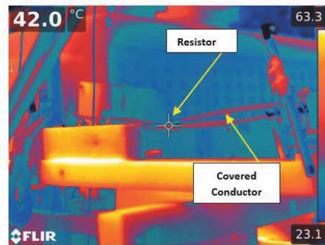
11:18 AM Energized –Test Subject Temp.: 42.0°C
