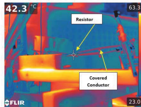
11:14 AM Energized –Test Subject Temp.: 42.3°C
