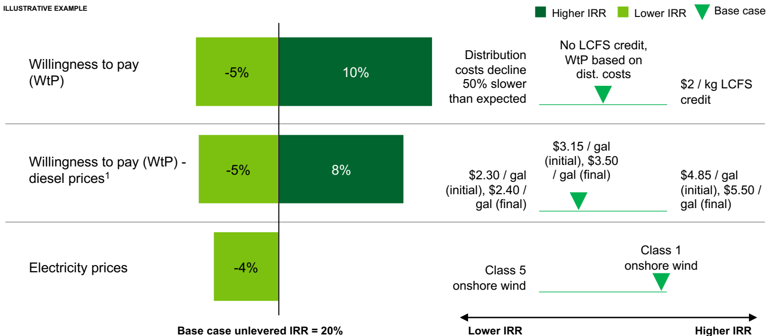
Figure 38: Sensitivities for project economics of hydrogen production with alkaline electrolysis for fuel cell truck off-takers
