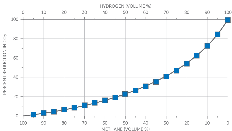
Figure 5: Relationship between CO 2 emissions and hydrogen/methane fuel blends (volume %).
