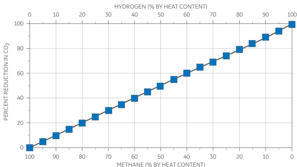
Figure 6: Relationship between CO 2 emissions and hydrogen/methane fuel blends (% heat input).
