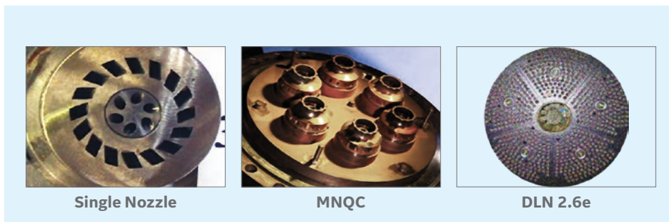
Figure 8: High hydrogen combustion systems.
