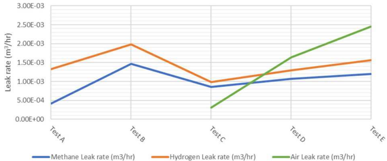
Figure 20: Measured leak rates for all test in the Hy4Heat project (93)
