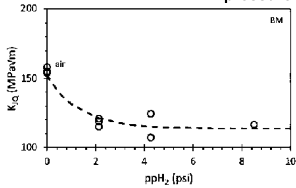
(a) base metal
