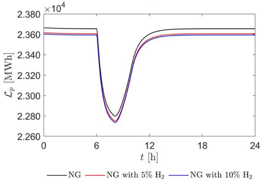
Figure 18: Simulated linepack for natural gas hydrogen blended natural gas at 5% and 10% (77)
