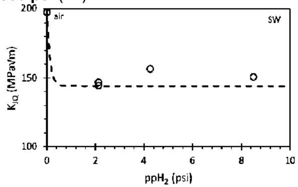
(b) seam weld
