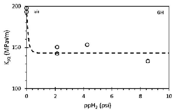
(e) girth HAZ
