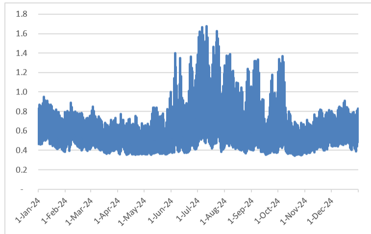
Figure 1. PG&E’s Representative Residential Customer Hourly Load, 2024 (kWh)
