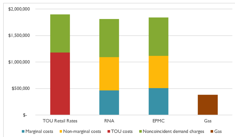
Figure 5. Fruit and Vegetable Canning Monthly Electric Costs from Incremental Thermal Battery Load, RNA vs EPMC
