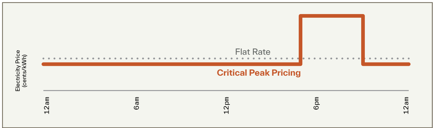
Figure 14. Critical Peak Pricing (on Event Day).
