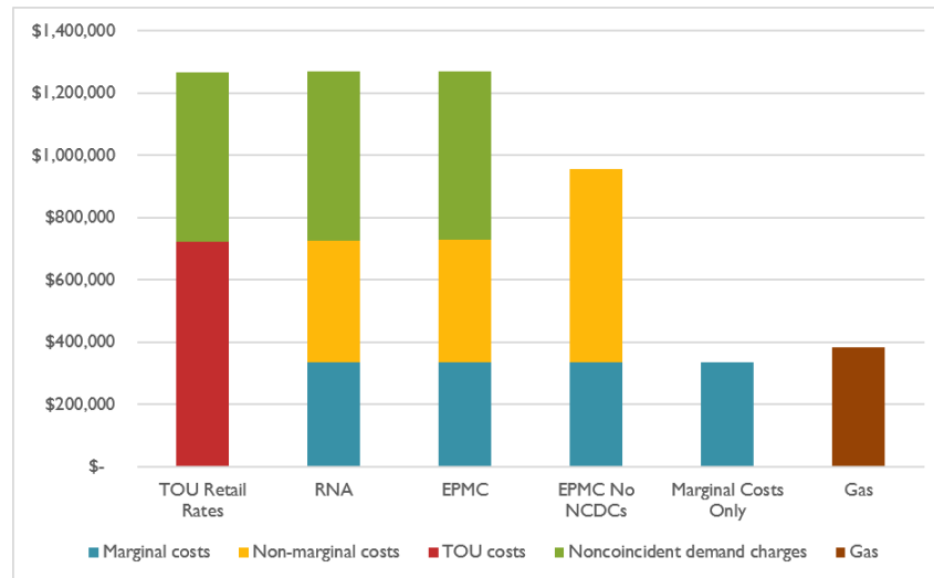
Figure 14. Pharmaceutical Manufacturing Monthly Electric Costs from Incremental Heat Pump Load
