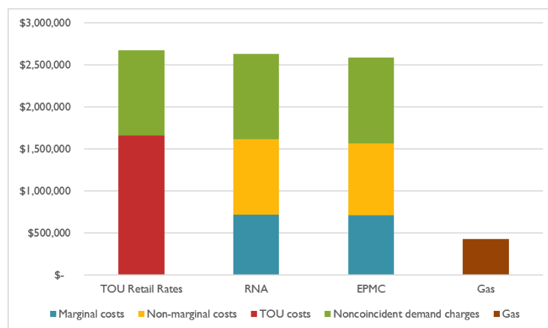
Figure 6. Pharmaceutical Manufacturing Monthly Electric Costs from Incremental Thermal Battery Load, RNA vs EPMC
