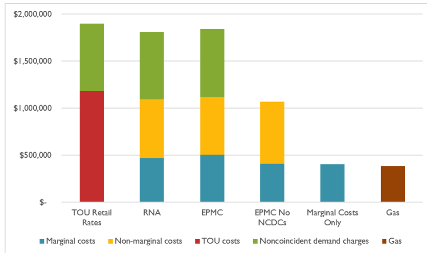
Figure 11. Fruit and Vegetable Canning Monthly Electric Costs from Incremental Thermal Battery Load, Marginal Costs Only
