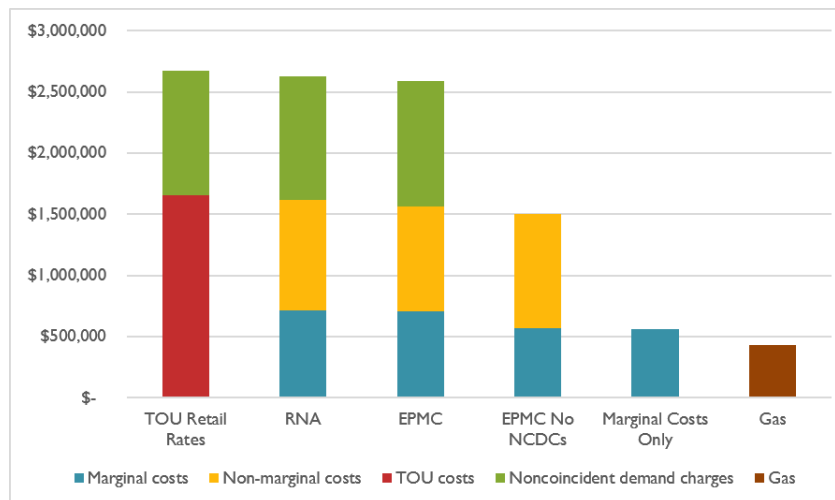
Figure 12. Pharmaceutical Manufacturing Monthly Electric Costs from Incremental Thermal Battery Load, Marginal Costs Only
