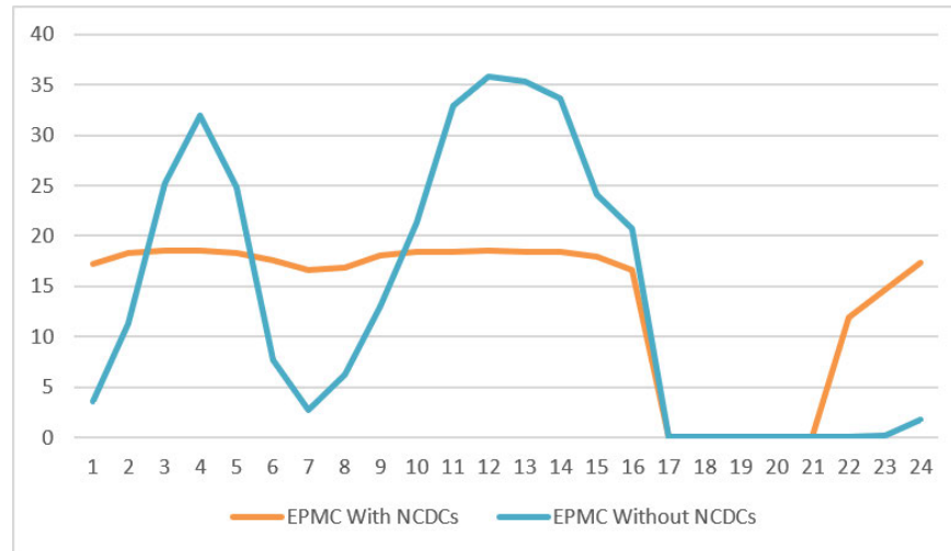
Figure 9. Fruit and Vegetable Canning Thermal Battery Average Weekday Load Profile (MW)
