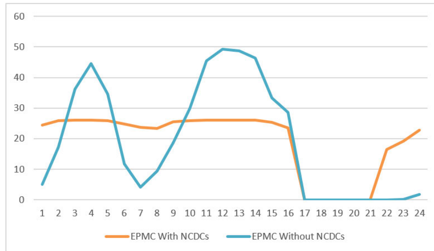
Figure 10. Pharmaceutical Manufacturing Thermal Battery Average Weekday Load Profile (MW)
