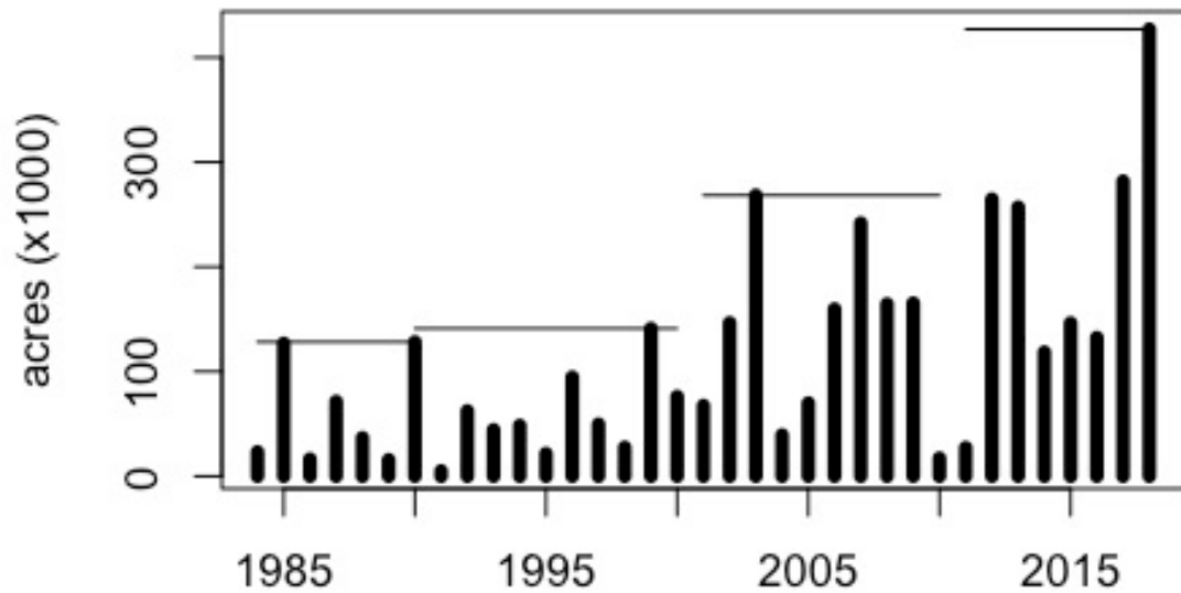
Figure III-17 Largest Annual Recorded Fire Size in California 1984-2018 80
