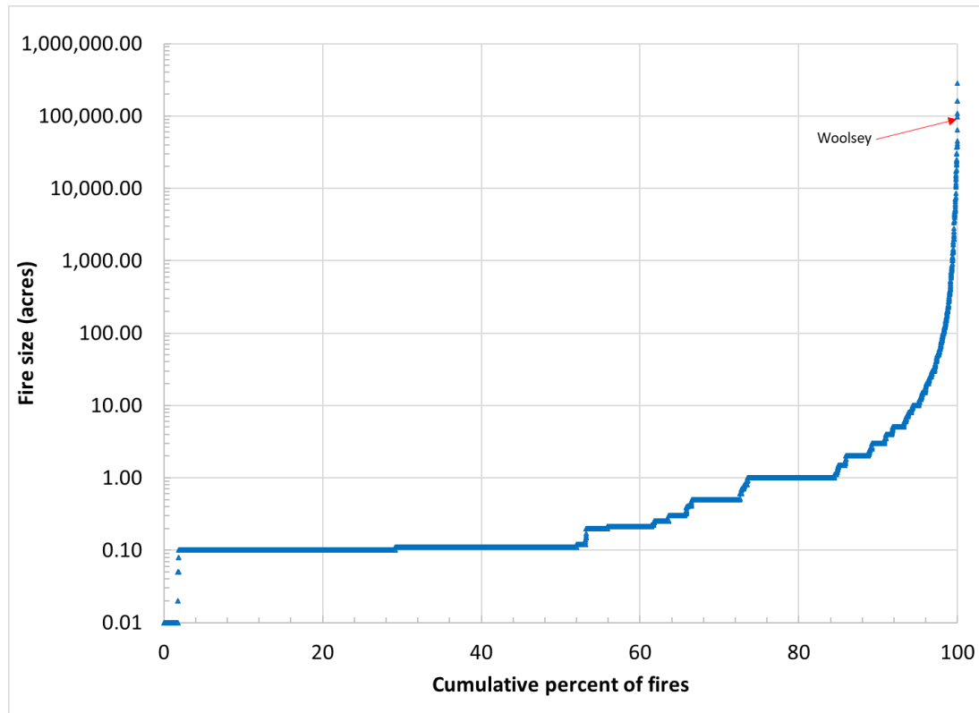
Figure D-1 Distribution of Fire Sizes for Fires Ignited in Los Angeles and Ventura Counties from 1992-2018 per FOD
