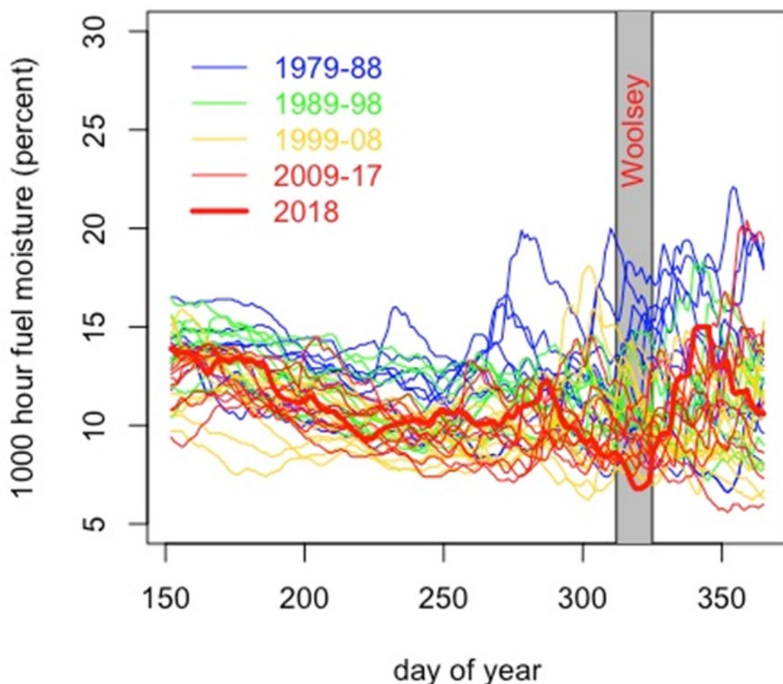
Figure III-20 1979-2018 Daily Fuel Moisture at Woolsey Fire Location
