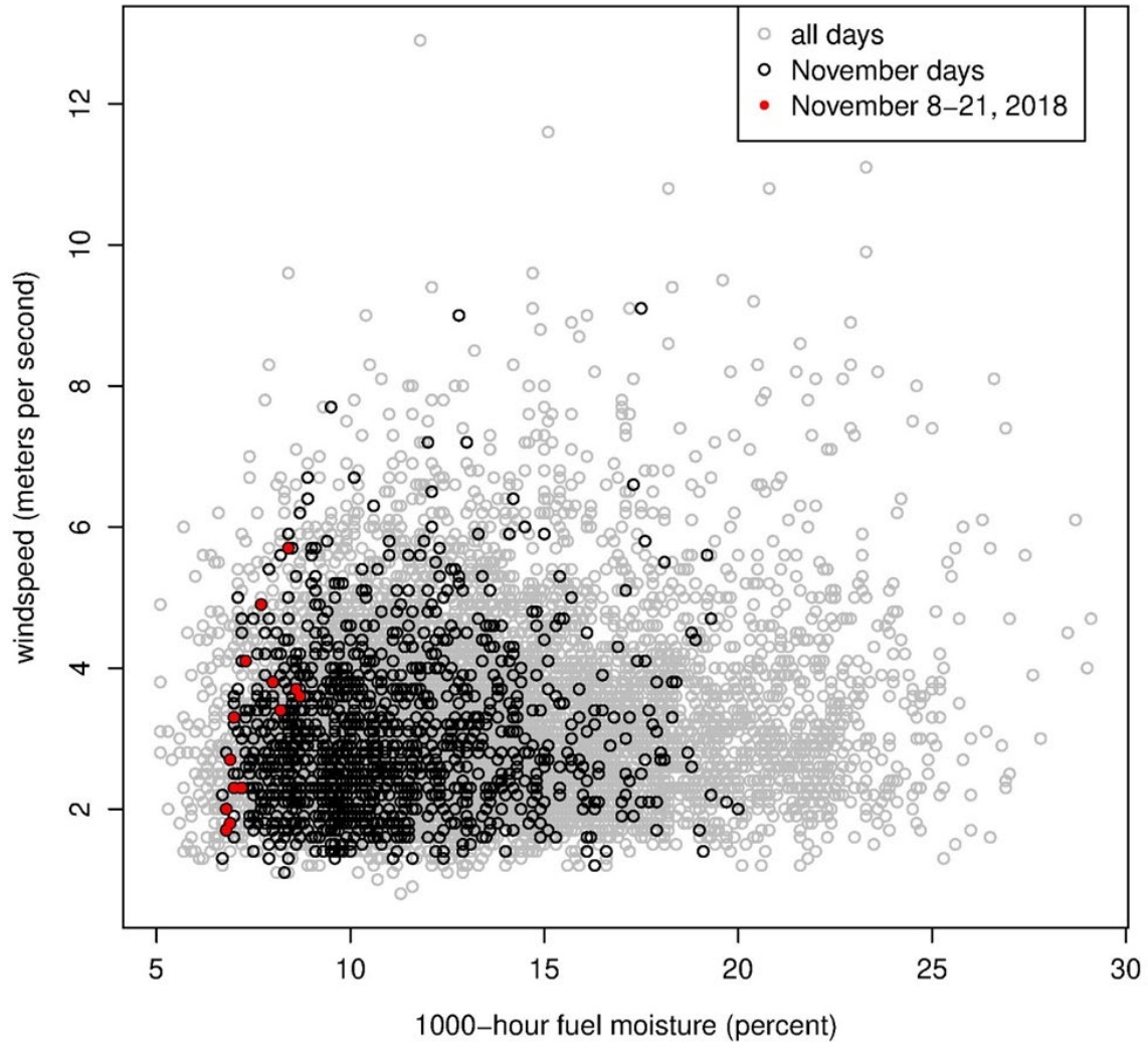
Figure III-19 Daily Maximum Windspeed vs. Estimated Daily Fuel Moisture at Woolsey Fire Location, 1984 – 2018
