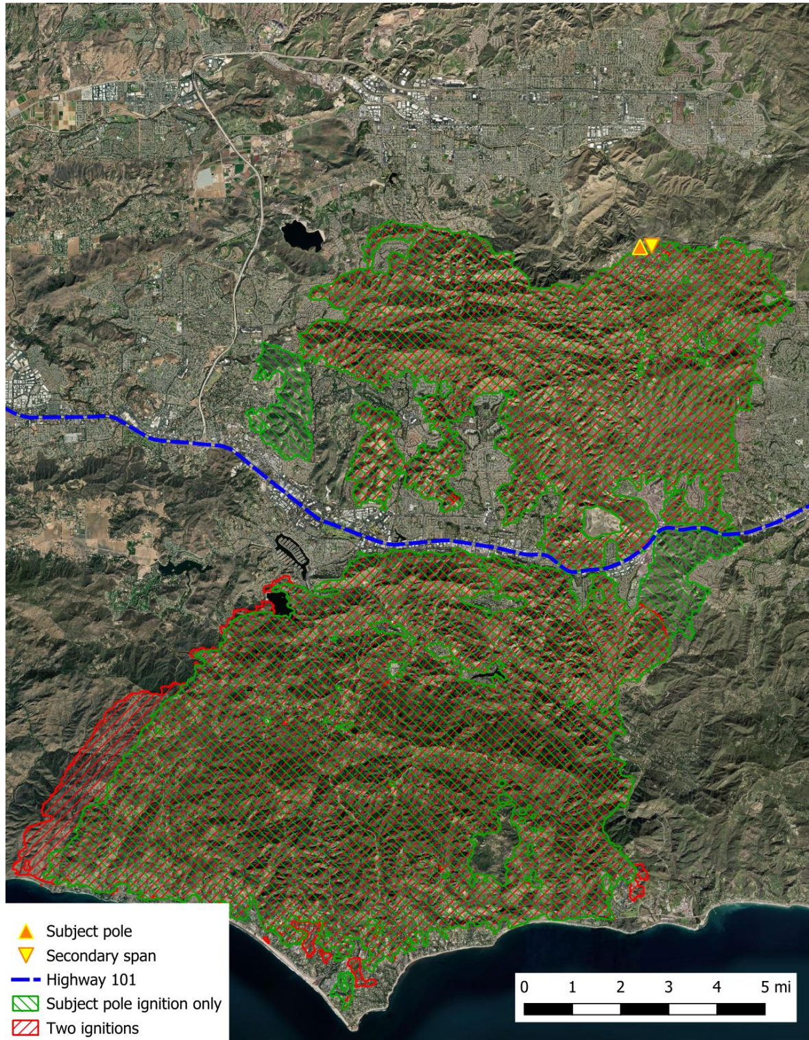
Figure II-14 Modeled Unsuppressed Fire Progression as of 1 p.m. on November 9, 2018 for Two Simultaneous Ignitions and Single Ignition 76
