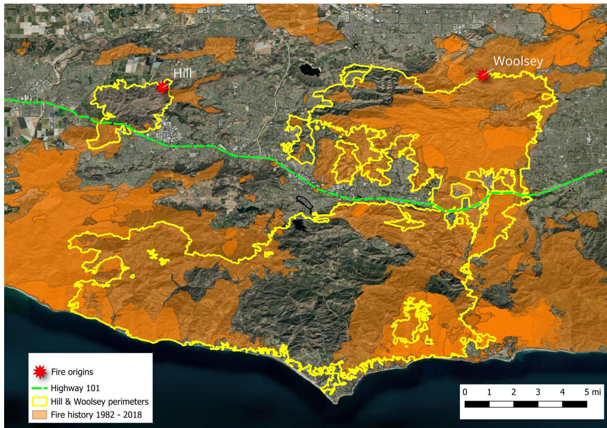
Figure II-10 Fire History (1982-2018) in the Hill & Woolsey Fire Footprints
