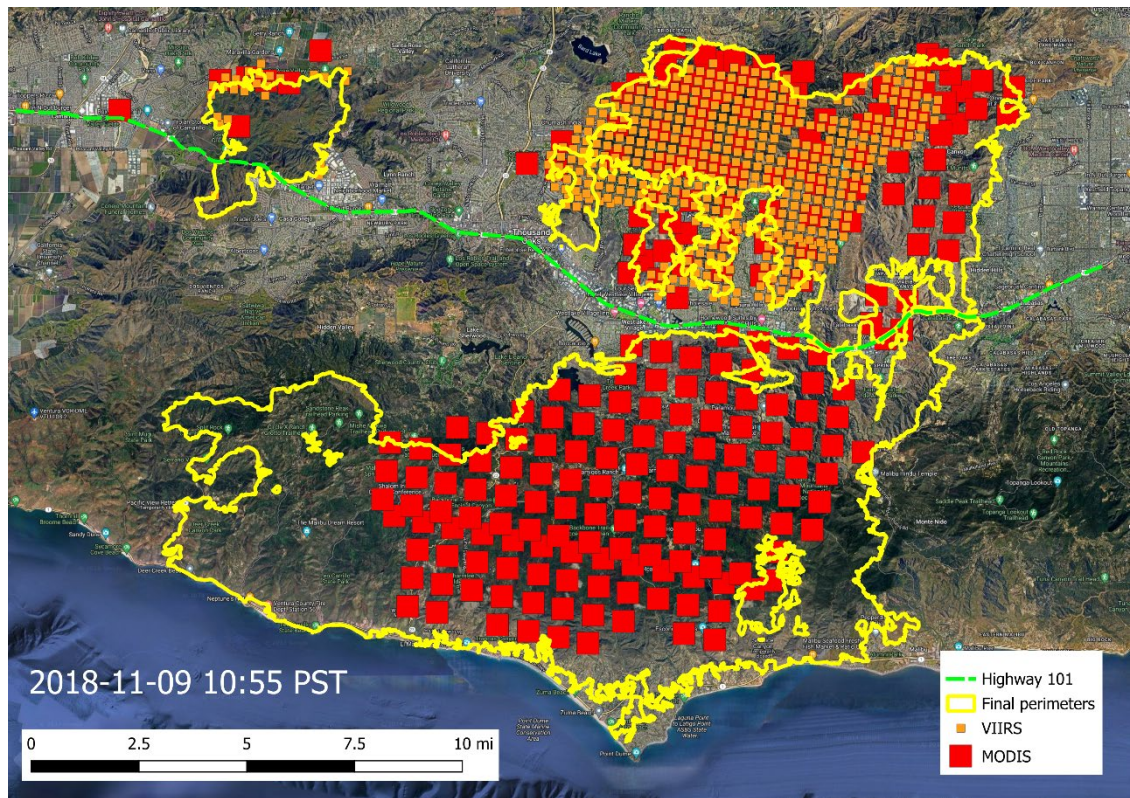
Figure II-12 MODIS & VIIRS Fire Hot Spots at 10:55 a.m. on November 9, 2018
