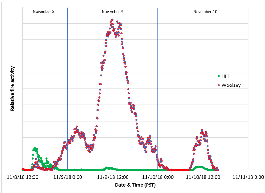
Figure II-7 Relative Fire Activity on Hill & Woolsey Fires from November 8-10, 2018
