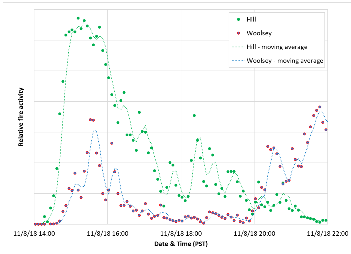
Figure II-6 Relative Fire Activity on Hill & Woolsey Fires on November 8, 2018
