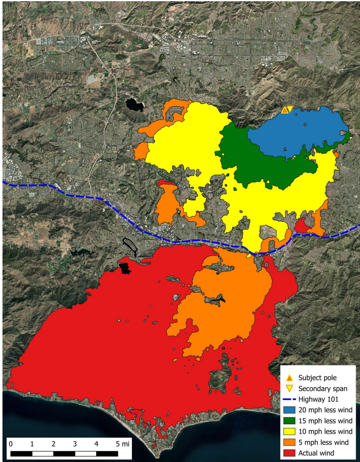
Figure II-13 Modeled Unsuppressed Fire Progression as of 1 p.m. on November 9, 2018 Under Different Wind Scenarios
