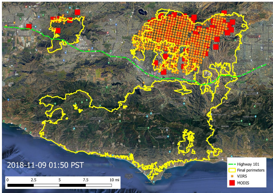
Figure II-11 MODIS & VIIRS Fire Hot Spots at 1:50 a.m. on November 9, 2018
