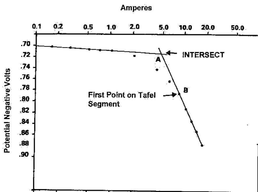
FIGURE B2—Sample E-Log-I Plot
